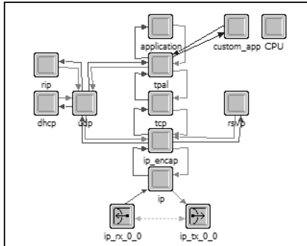
Figure 7. Modified workstation model [15].
