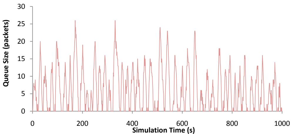
Figure 49. Actual queue size controlled by the controller model. Poisson traffic, 10 second sample period, grey line: actual queue size.
