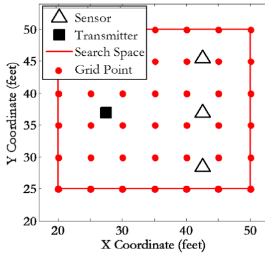
Figure 17: Example node localization search space
