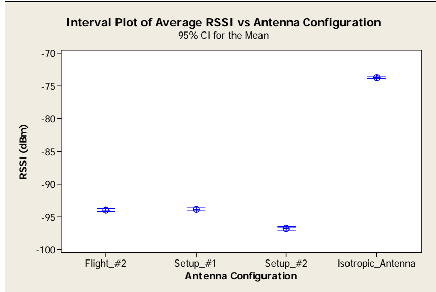
Figure 26: Interval Plot of RSSI vs Antenna (Flight #2)
