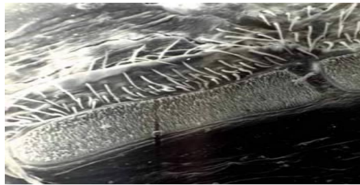
Figure 2. Cribellum Organ [59]
