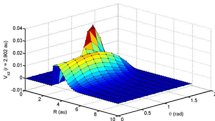
Figure 24. The diabatic coupling surface V_{xz} for r = 2.902 au calculated using the ADT mixing angle determined by the line integral starting at \theta = \pi/2 and ending at \theta = 0
