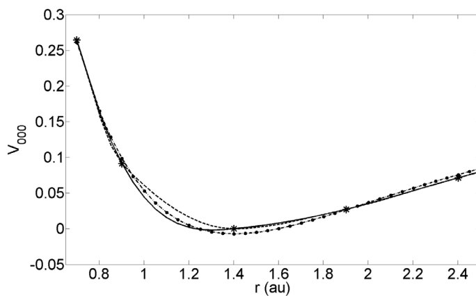
Figure 38. A comparison of three methods for fitting the H_2 PES in the asymptotic limit: cubic spline (solid), piecewise cubic Hermite (dashed), Morse fitting function (dash-dot), V_{000} data (asterisk)
