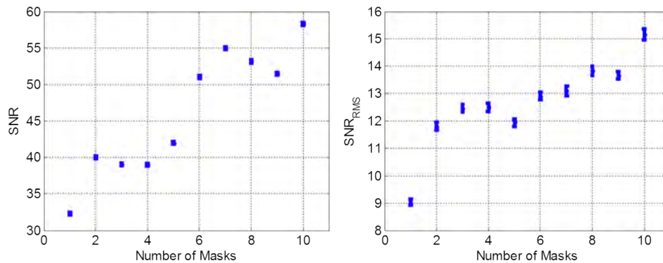
Figure 46. Left: SNR versus number of masks used, Cd-109 with background, 1 hr detection time. Right: SNR RMS versus number of masks used, Cd-109 with background, 1 hr detection time.
