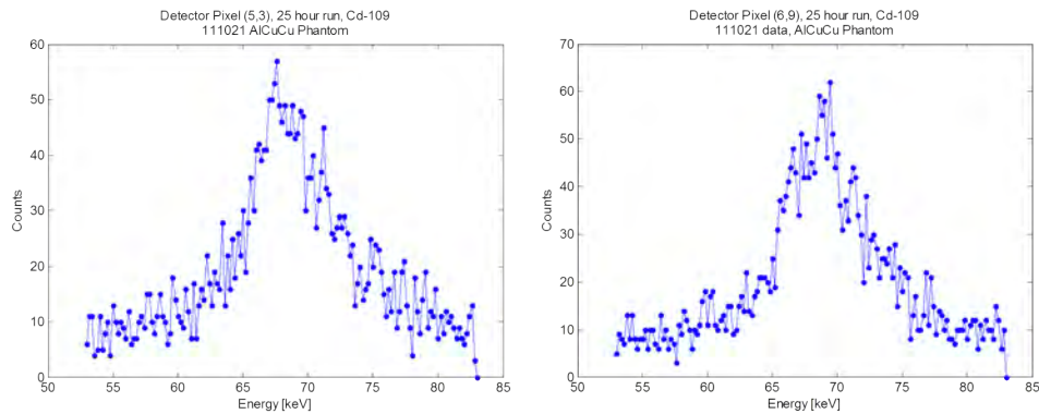
Figure 57. Spectra received from the AICuCu phantom, taken from two different detector pixels.
