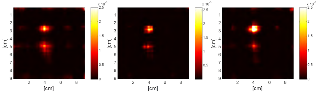
Figure 43. The effect of different energy windows. The colorscale is fixed. Left: 84-92 keV window. Center: 86-90 keV window. Right: 87-89 keV window.
