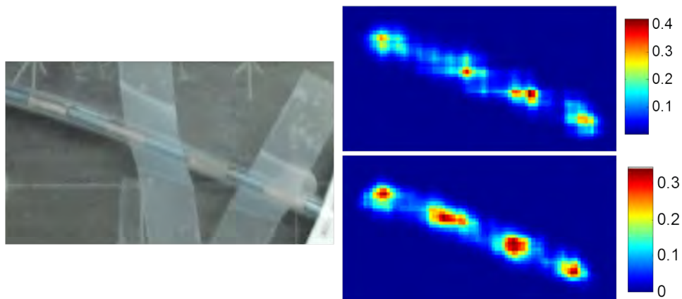
Figure 48. Left: Picture of the Rod. Top-Right: The ML-EM image reconstruction using 1 mask, zoomed. Bottom-Right: The ML-EM image reconstruction using 10 masks, zoomed.
