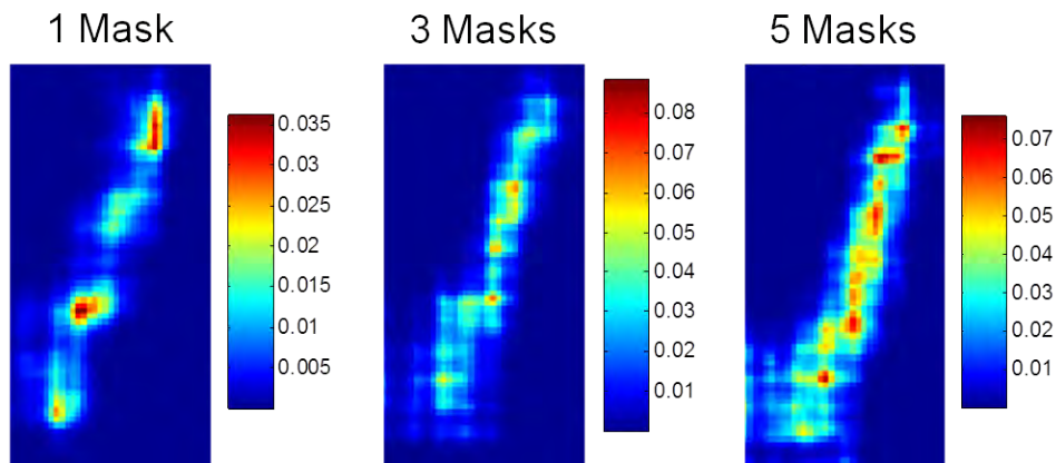
Figure 49. Zoomed view of the rope after 1, 3, and 5 masks, ML-EM, 150 iterations.
