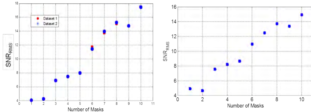
Figure 51. Left: \text{SNR}_{\text{RMS}} for the Co-57 button source, as a function of number of masks used, correlation decoding. Right: \text{SNR}_{\text{RMS}} for the Cd-109 source with background, as a function of number of masks used, correlation decoding.
