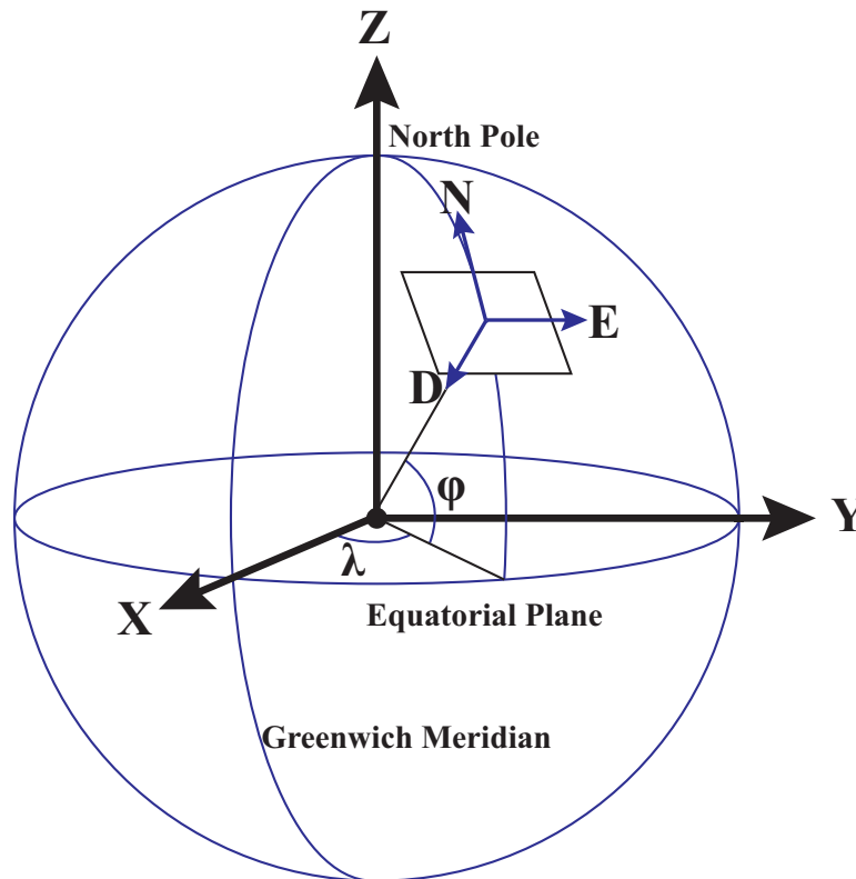
Figure 2. Diagram relating WGS84, ECEF and NED coordinate systems and their relationships. The graphic represents a simplified version of the WGS84 ellipsoid model. Black arrows are ECEF coordinates, and blue arrows are NED coordinate system centered at a specific location on the Earth.
