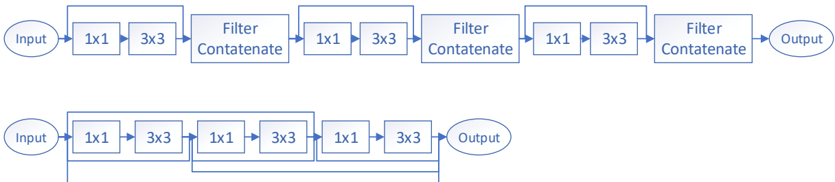
Figure 11. An example of a three composite function dense block from DenseNet. Top is the implementation, and the bottom displays the composite function's connectivity.
