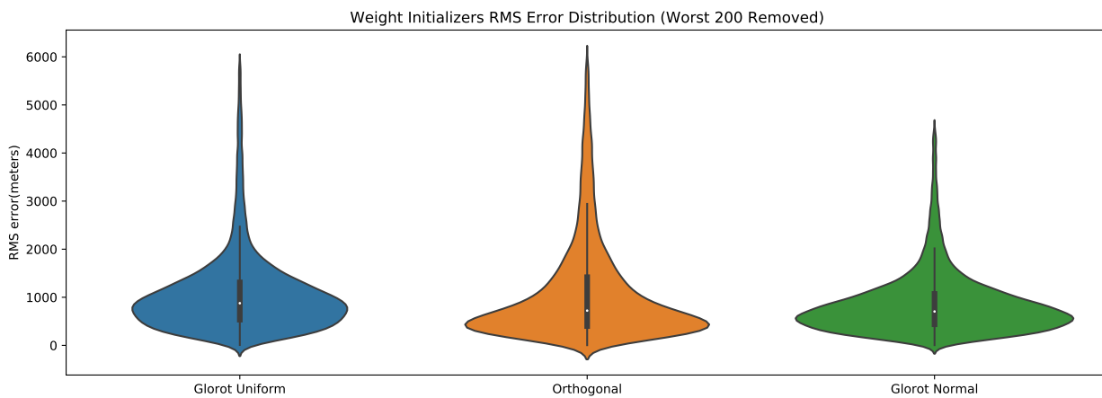
Figure 37. This violin plot displays the RMS error results of the test dataset for the weight initializer comparison models: Glorot uniform, orthogonal, and Glorot normal. Each model was trained for 50 epochs, and the worst 200 RMS errors were removed for readability.
