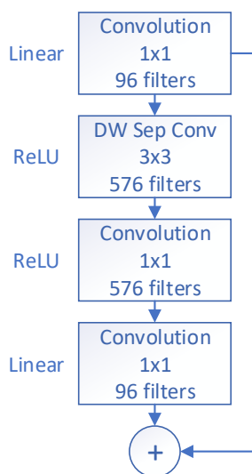
Figure 4. The MobileNet V2 inverted residual with linear bottleneck pulls the bottleneck layer (one that is designed to reduce filters) to the outside of the convolution layers. the linear activation of the bottleneck layers aids the network in retaining linearities because they are residually connected through non-linear layers.
