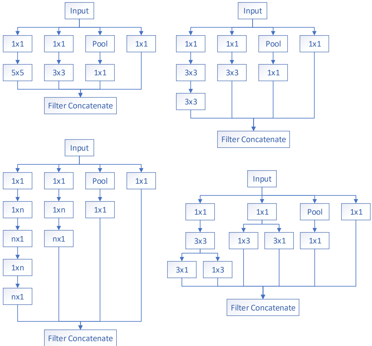
Figure 5. Inception Modules. Top left is the original Inception module. Top right has the 5 \times 5 convolution replaced with two 3 \times 3 convolutions. Bottom left is a middle layer where n = 7 , used to reduce computational complexity. Bottom right is a lower layer used to reduce computations of 3 \times 3 convolution.
