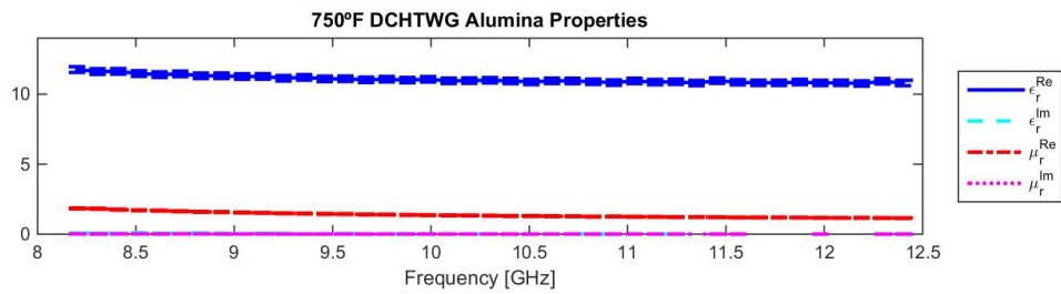
(c) Alumina 750°F analysis using DCHTGW
