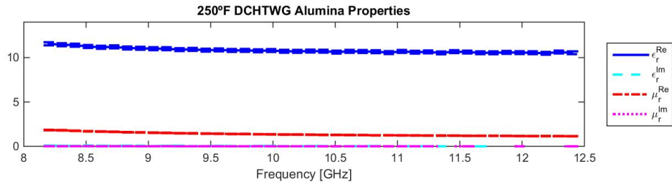
(a) Alumina 250°F analysis using DCHTGW
