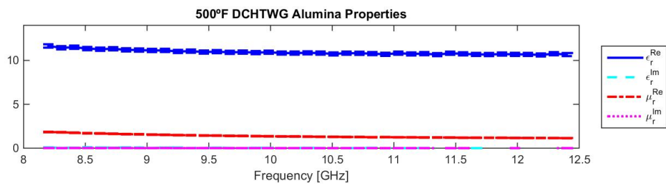
(b) Alumina 500°F analysis using DCHTGW
