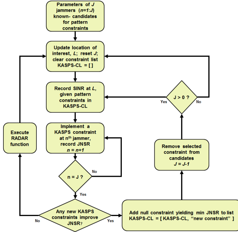
Figure 11. Flow diagram demonstrating how the subarray pattern nulling decision is algorithmically determined.
