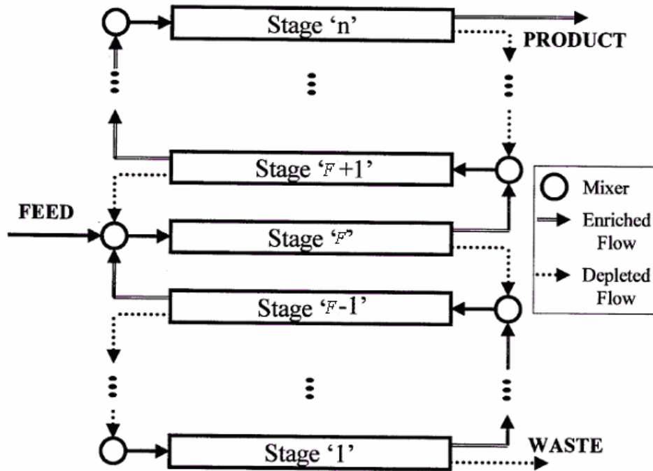
Figure 1. Example of 1 up-1 down Cascade
