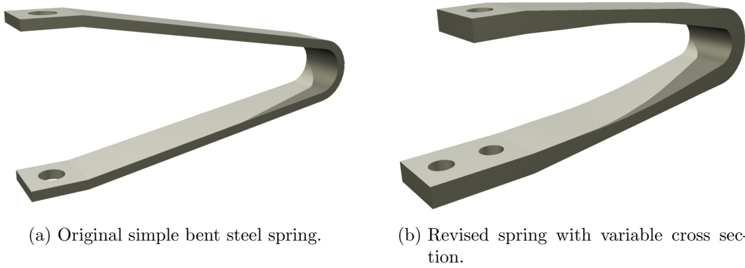
Figure 13 Changes in spring design from FE analysis
