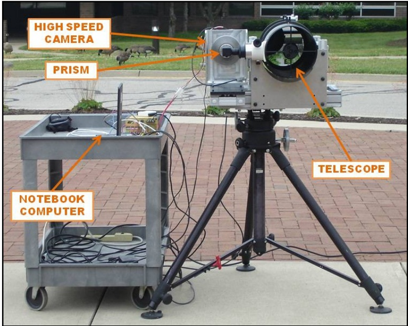
Figure 3 Photo of CTEEx ground based prototype [7]
