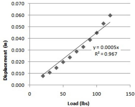
Figure 27 Lateral load test for stainless steel springs with linear regression
