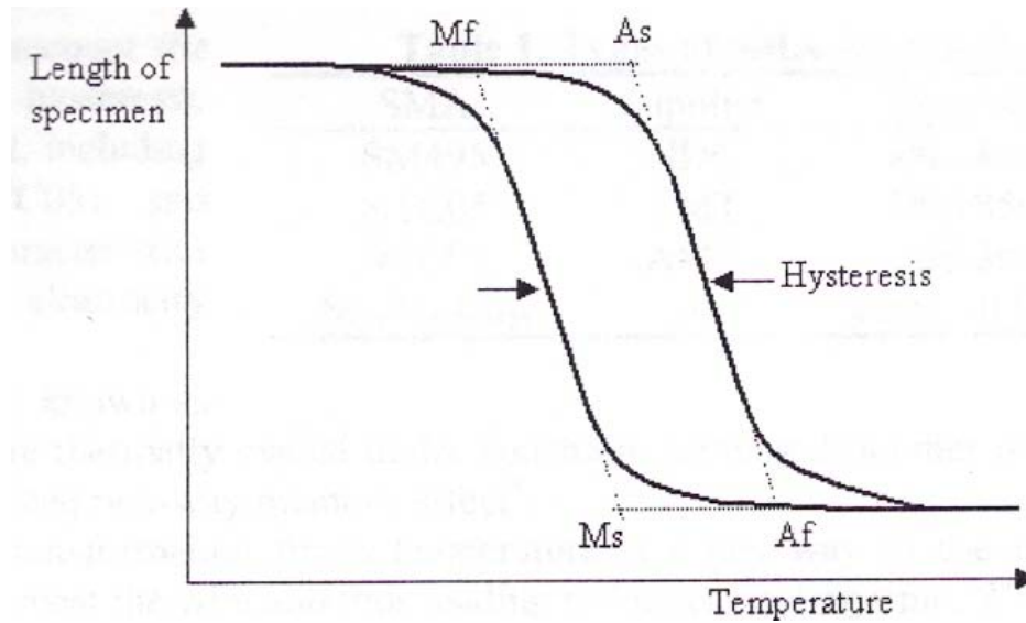
Figure 10. Wire Length Versus Temperature (Seow and Liu, 2008:2)
