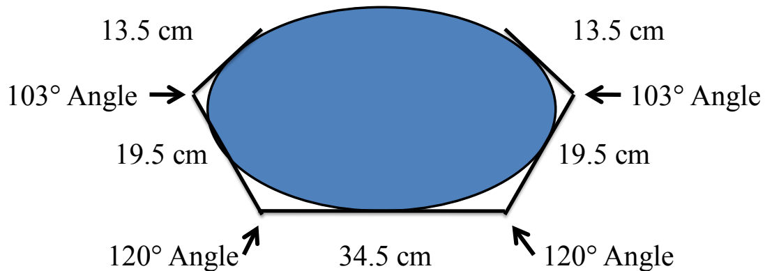
Figure 47. Mod-2 Dimensions
