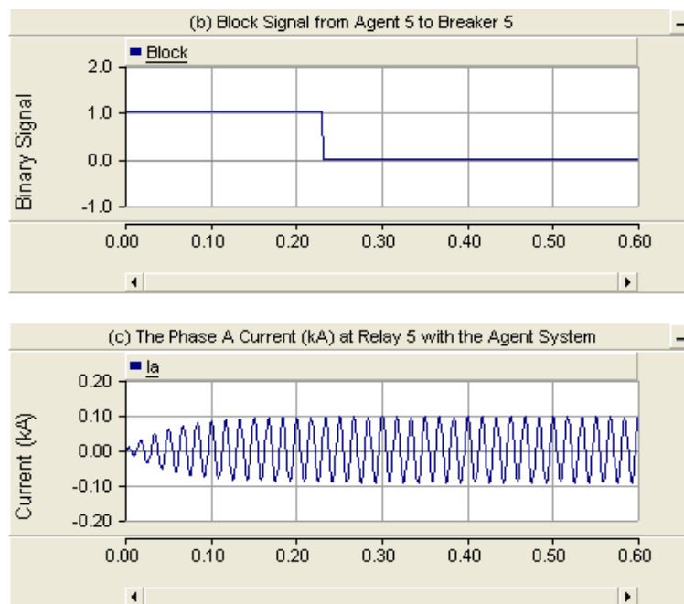
Figure 14. Correct blocking of false trip signal with the trust system. When a false trip signal was sent to Breaker 5 at 0.20 seconds, Agent 5 is rapidly able to block Breaker 5 from tripping using information from trusted agents to ensure the current continued to flow.
