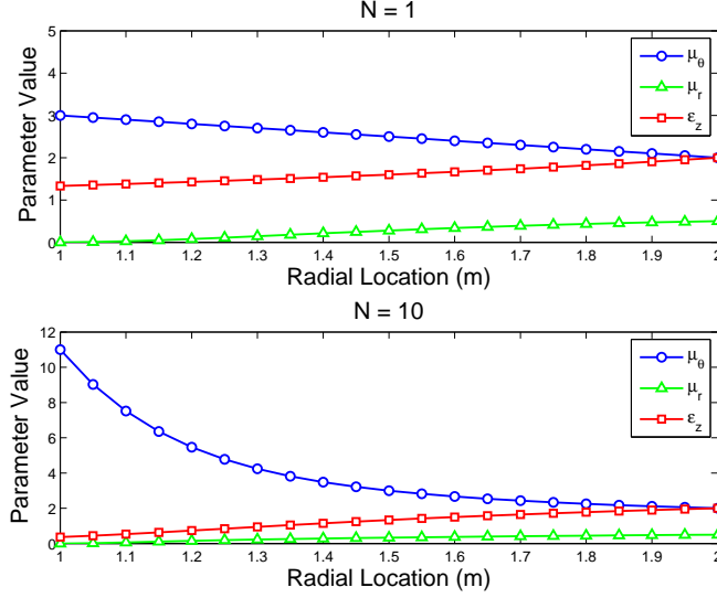
Figure 4.14: Parameter variation as a function of r . In both figures, the \circ -line is \mu_\theta , the \Delta -line is \mu_r , and the \square -line is \epsilon_z . In the top figure \mu_\theta is approximated using N = 1 ; in the bottom figure, N = 10 .
