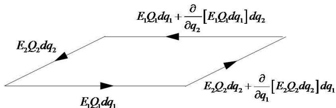
Figure A.2: Line integral differential components
