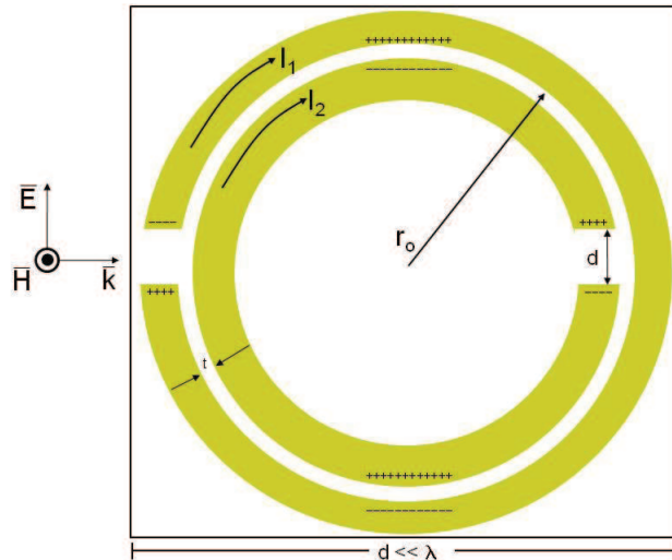
Figure 3.4: Edge Coupled Split Ring Resonator
