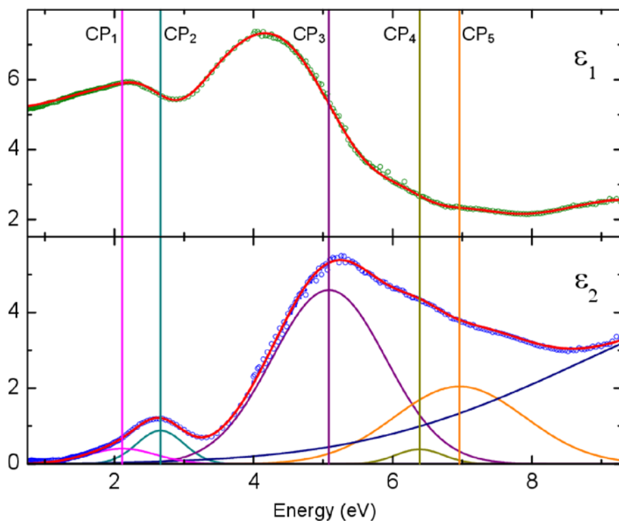
Figure 32. The real and imaginary parts of the \text{UO}_2 dielectric function extracted from the variable angle spectroscopic ellipsometry by wavelength-by-wavelength analysis (green and blue circles, respectively) shown in comparison with the critical point model dielectric function (red solid). Individual contributions to the imaginary part of the dielectric function obtained with Gaussian oscillators are shown with vertical lines corresponding to their center energies (CP 1 -magenta, CP 2 -dark cyan, CP 3 -violet, CP 4 -dark yellow, CP 5 -orange, as well as another contribution outside the investigated spectral range to account for higher energy transitions shown as navy).
