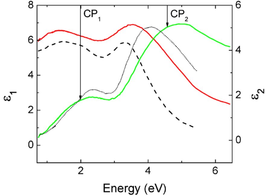
Figure 20. Dielectric function of single-crystal \text{UO}_2 obtained in this analysis (red and green solid lines, respectively) compared to those by Siekhaus et al. [36](black dash and dot, respectively). Both the results of Siekhaus et al. [38] and this work come from ellipsometric techniques (see text). Arrows indicating the critical points identified by our work are labeled and correspond to Gaussian oscillator parameters.
