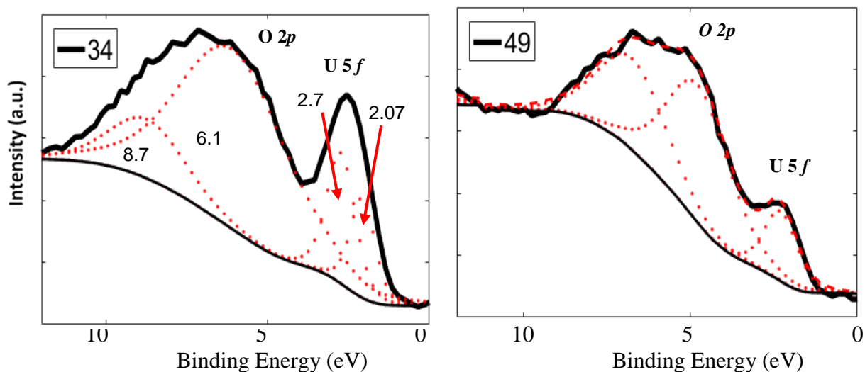
Figure 30. The O 2p and U 5f binding energies are peak deconvolved for 34 and 49^\circ respectively. The dotted red lines represent the individual deconvoluted peaks, while the red dashed line is the summation of the peak deconvolution. The 34^\circ spectrum provides evidence of the spin orbit coupled U 5f_{7/2} and U 5f_{5/2} orbitals while in the 49^\circ spectrum the U 5f orbitals are indistinguishable.
