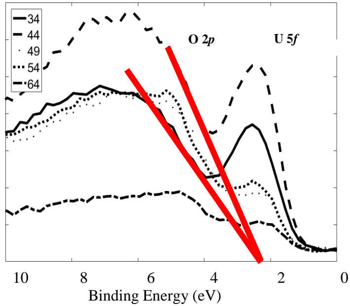
Figure 29. The AR-XPS spectra for the UO 2 valence band edge collected for angles of 34, 44, 49, 54, and 64° between the surface and the x-ray source. An electronic band gap of ~2.2 eV is denoted by red lines.
