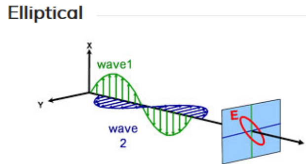
Figure 7. Two electromagnetic waves traveling orthogonal to the direction of propagation with arbitrary amplitude and phase [13].
