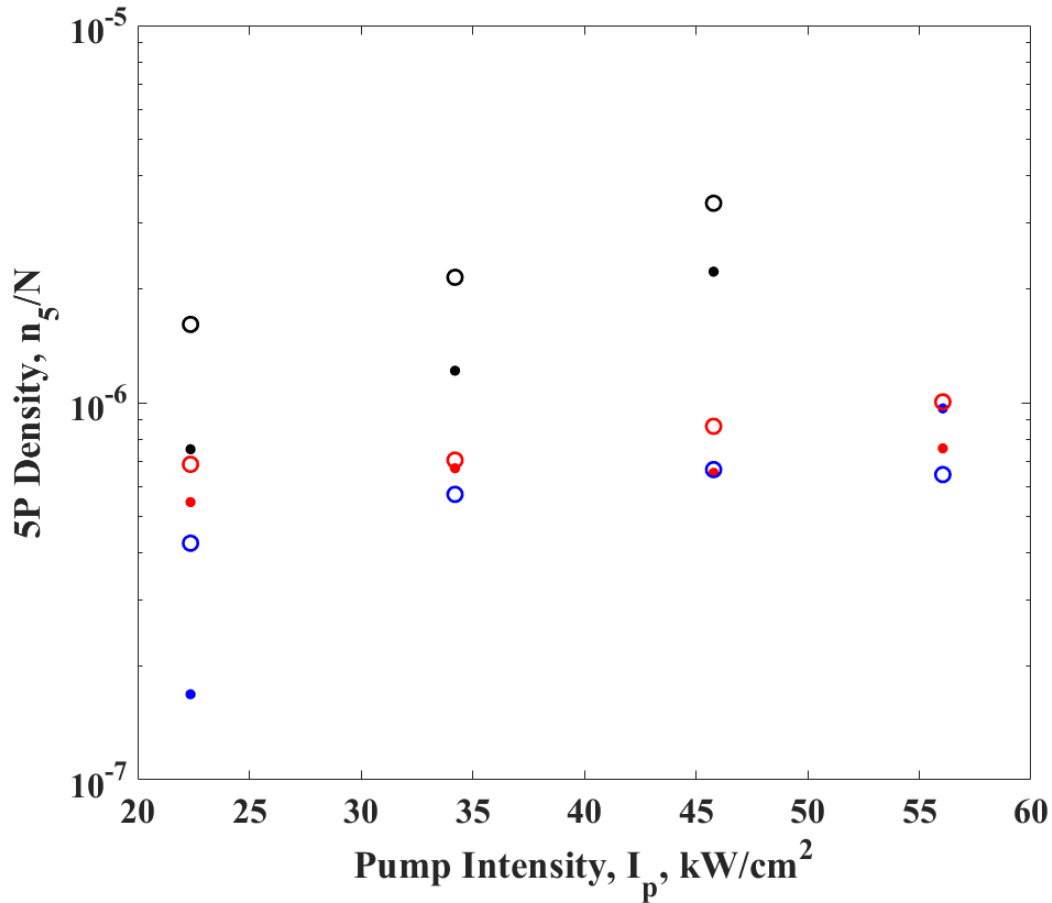
Figure 56. The observed ( \bullet ) and predicted ( \circ ) density in the 5^2P state as a function of pump intensity in a 6.7% methane buffer gas, in the presence of very weak lasing, I_l = 100 W/cm^2 . The black dots represent N \sim 1 \times 10^{13} cm^{-3} , P= 450 Torr, red is N \sim 5 \times 10^{13} cm^{-3} , P= 450 Torr, and blue has N \sim 6 \times 10^{13} cm^{-3} , P= 850 Torr.
