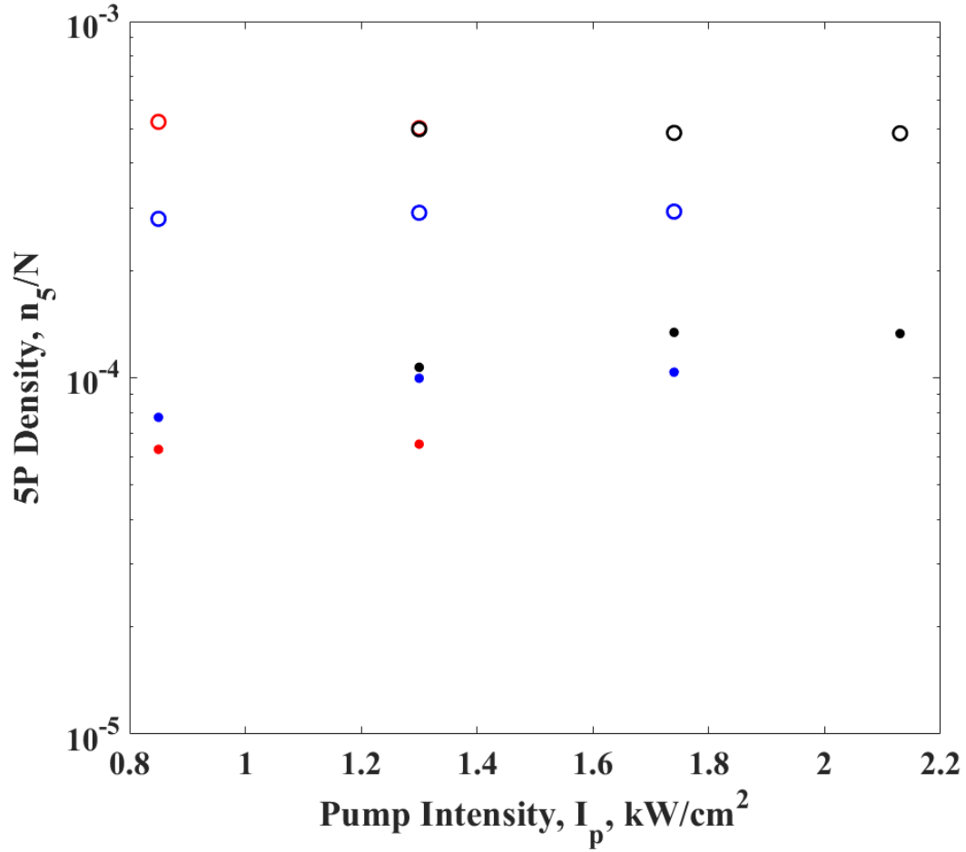
Figure 49. The observed ( \bullet ) and predicted ( \circ ) density in the 5^2P state as a function of pump intensity at N \sim 1 \times 10^{14} \text{ cm}^{-3} with helium pressures of P=850 (blue) without lasing, and P=450 with (red) and without (black) lasing. The model presented in (80) is used to calculate the intermediate prediction.
