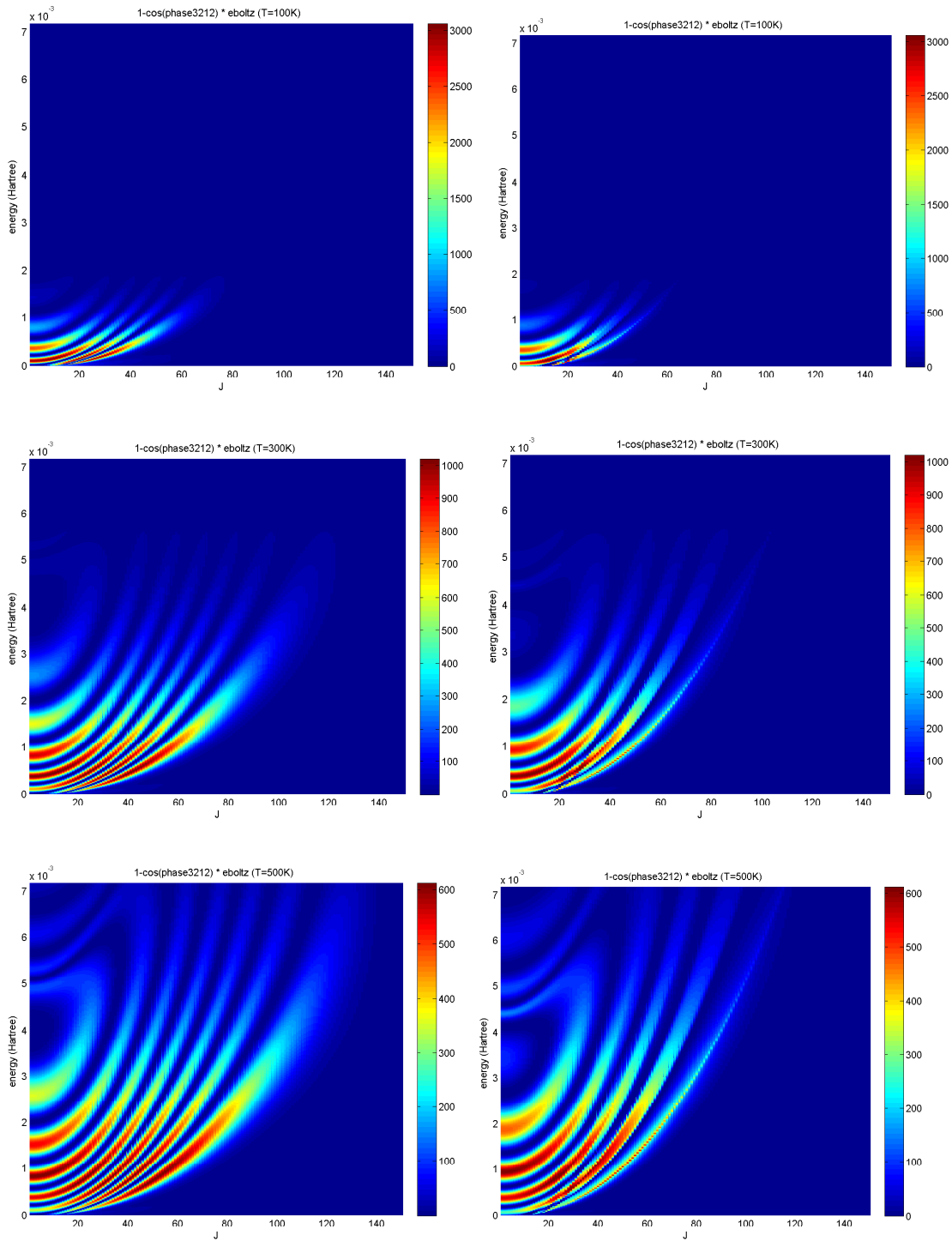
Fig. 3.10.3b: [1 - \cos \theta_j(E)] \times Boltzmann distribution for the \left| \frac{3}{2}, \frac{1}{2} \right\rangle state of the uncoupled case (left) and the fully-coupled 3x3 case (right) of Cs + He at T = 100 K (top), 300 K (middle), and 500 K (bottom), top-down view.
