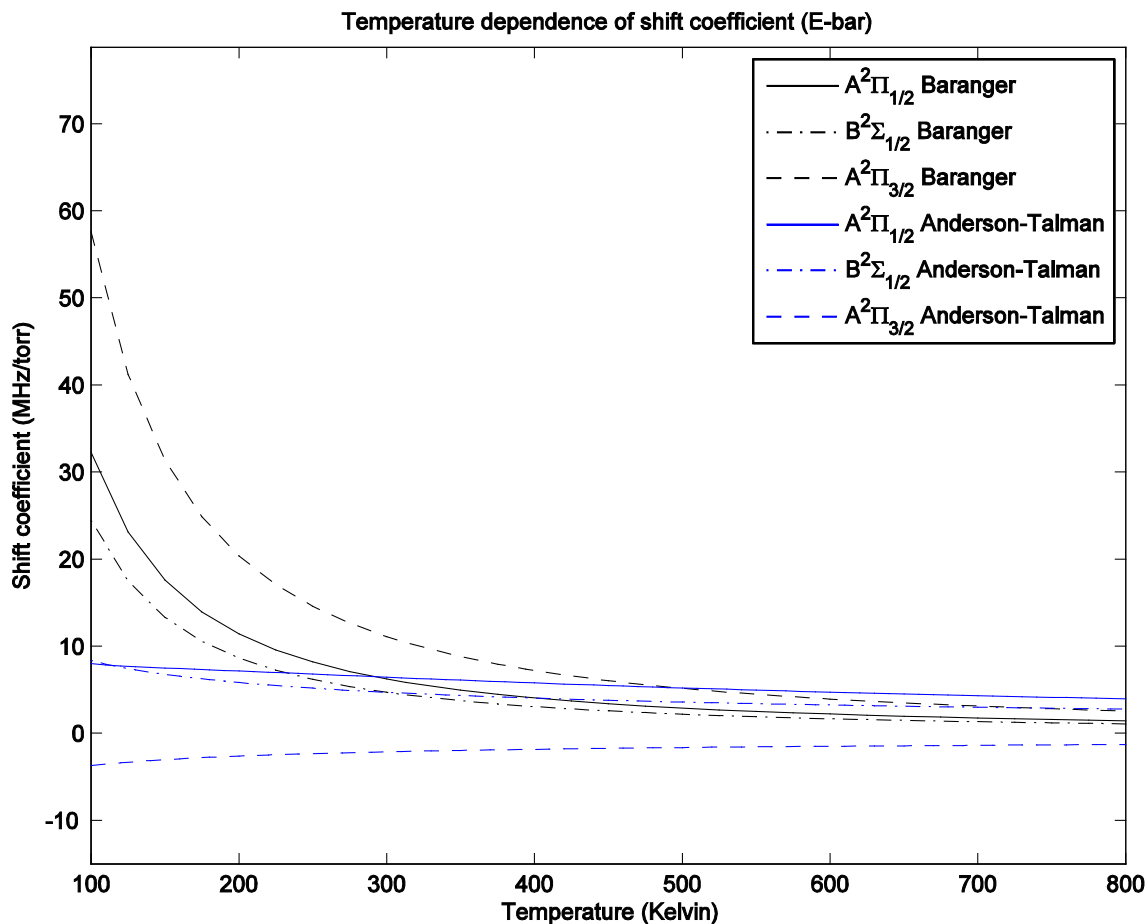
Fig. 2.51: Shift coefficients vs. temperature for Rb + He, uncoupled, average kinetic energy
