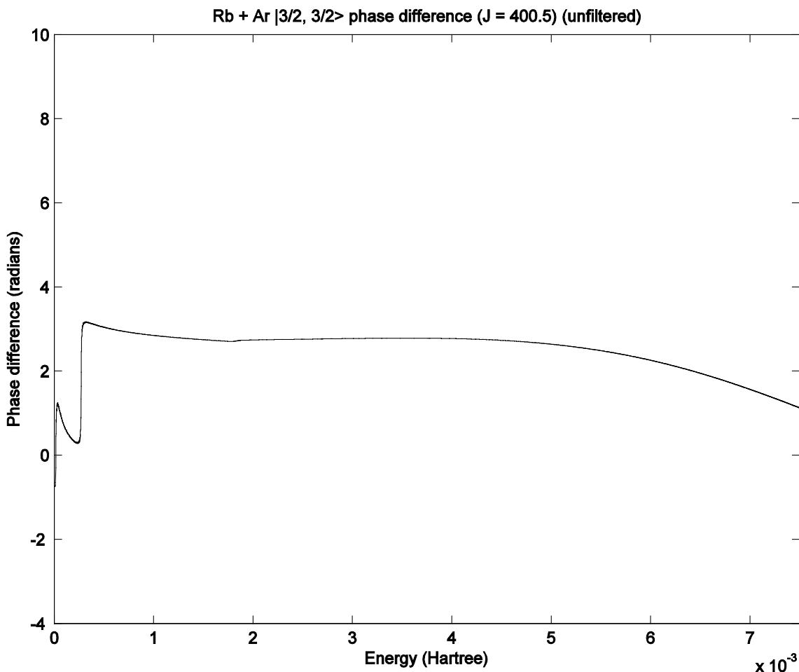
Fig. 3.10.2c: Scattering phase shift difference for the A^2\Pi_{3/2} state, at J = 400.5 , in the coupled case of Rb + Ar, before filtering. The “shelf” that appears at the low-energy edge of Fig. 3.10.2b can be seen at the left end of this plot and is caused by “divide by zero error”. An overall phase difference offset is a computational artifact created by the choice of a nonzero phase at J = 0.5 , E = 0 and represents the separation of the medium-energy portion of this plot from zero phase difference. A third source of error (at higher energies) is caused by Moller state limitations.
