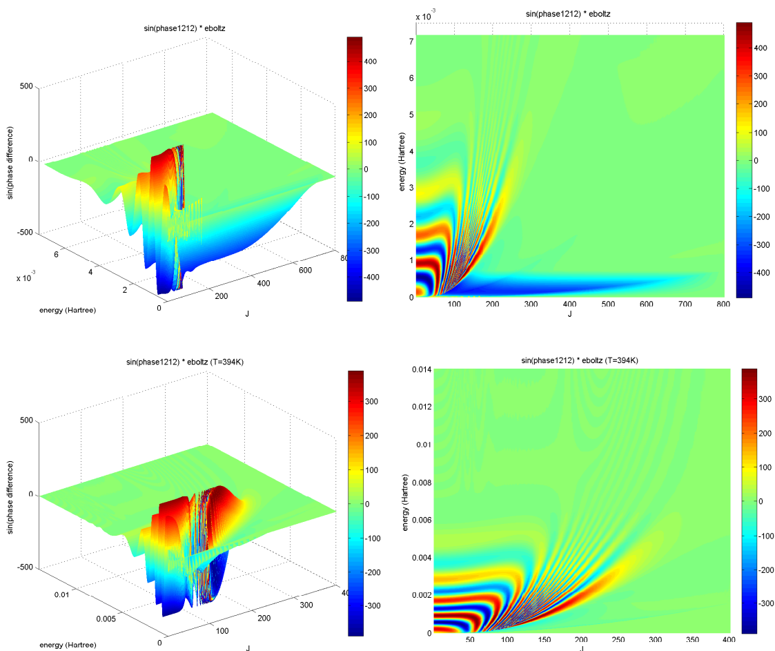
Fig. 3.10.2h: \sin \theta_j(E) \times Boltzmann distribution for the A^2\Pi_{1/2} state of the uncoupled case of Cs + Ar, at T = 394 K, side view (left) and top-down view (right). An early attempt (top) at generating the Moller states proved not to propagate far enough into the distant past. The latest run (bottom) propagates twice as far. Note that there are differences in scale between the runs. The feature appearing across the low-energy edge of the early run (top) is caused by the Moller state issue. Moller states in both data sets satisfied all the needs of the work of Lewis (Lewis, 2011), but give wholly inadequate scattering phase shift differences.
