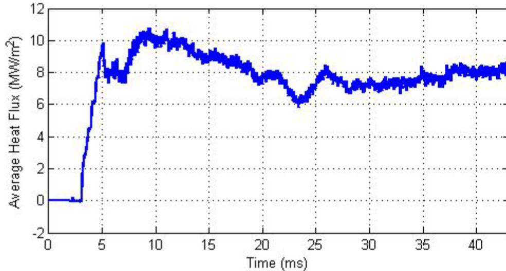
Figure 25. Average heat flux into the gauge
