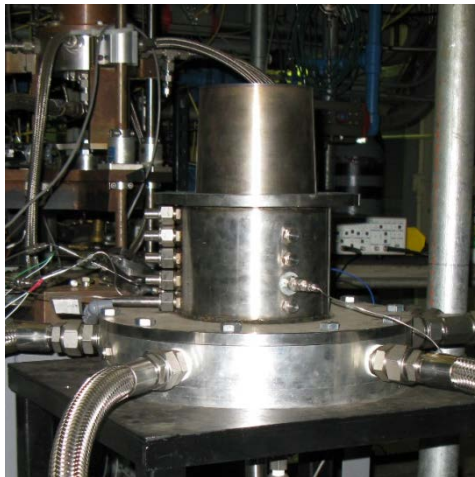
Figure 16. Modified 6-inch RDE used for heat flux gauge testing
