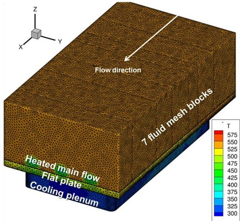
Figure 23 – Flat plate 3-D CHT CFD theoretical and actual computational domain extents featuring boundary condition tagging (top) and basic temperature contours [K] (bottom).
