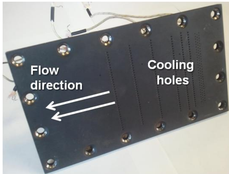
Figure 40 – Image of the baseline cooled flat plate hot flow side.
