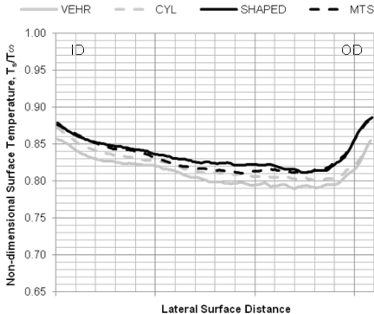
Figure 134 - Spanwise (lateral) non-dimensional surface temperature for the four different hole shapes on the optimized flat plate RTV PS cooling array at the leading edge location.
