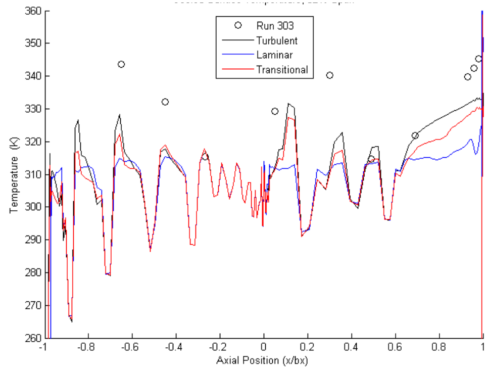
Figure B.11 - Comparison of CEEF CFD predictions using T_{\infty,nw} and TRF experimental cooled vane surface temperature at 62% span.
