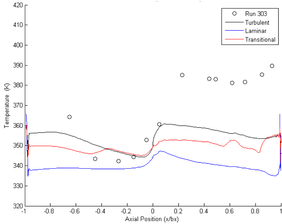
Figure B.5 - Comparison of CEEF CFD predictions using T_{\infty,nw} and TRF experimental uncooled vane surface temperature at 62% span.
