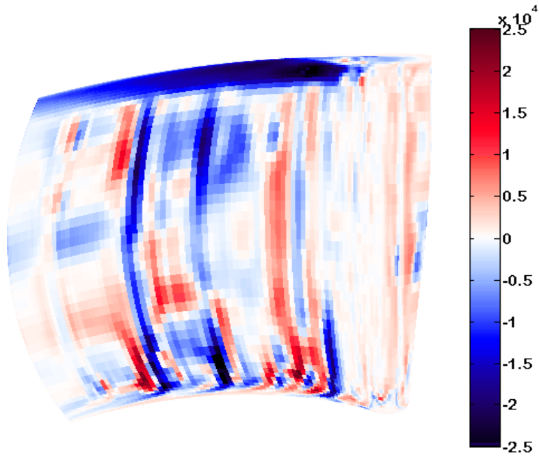
Figure 80 - PS contour of near-wall (q''_{\text{optimized}} - q''_{\text{baseline}}) [ \text{W/m}^2 ]. Flow goes from right to left.
