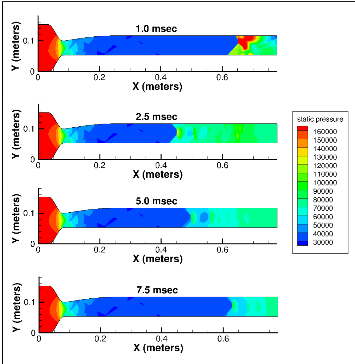
Figure 23. Evolution of PCST solution for instant 75.0 kPa back pressure
