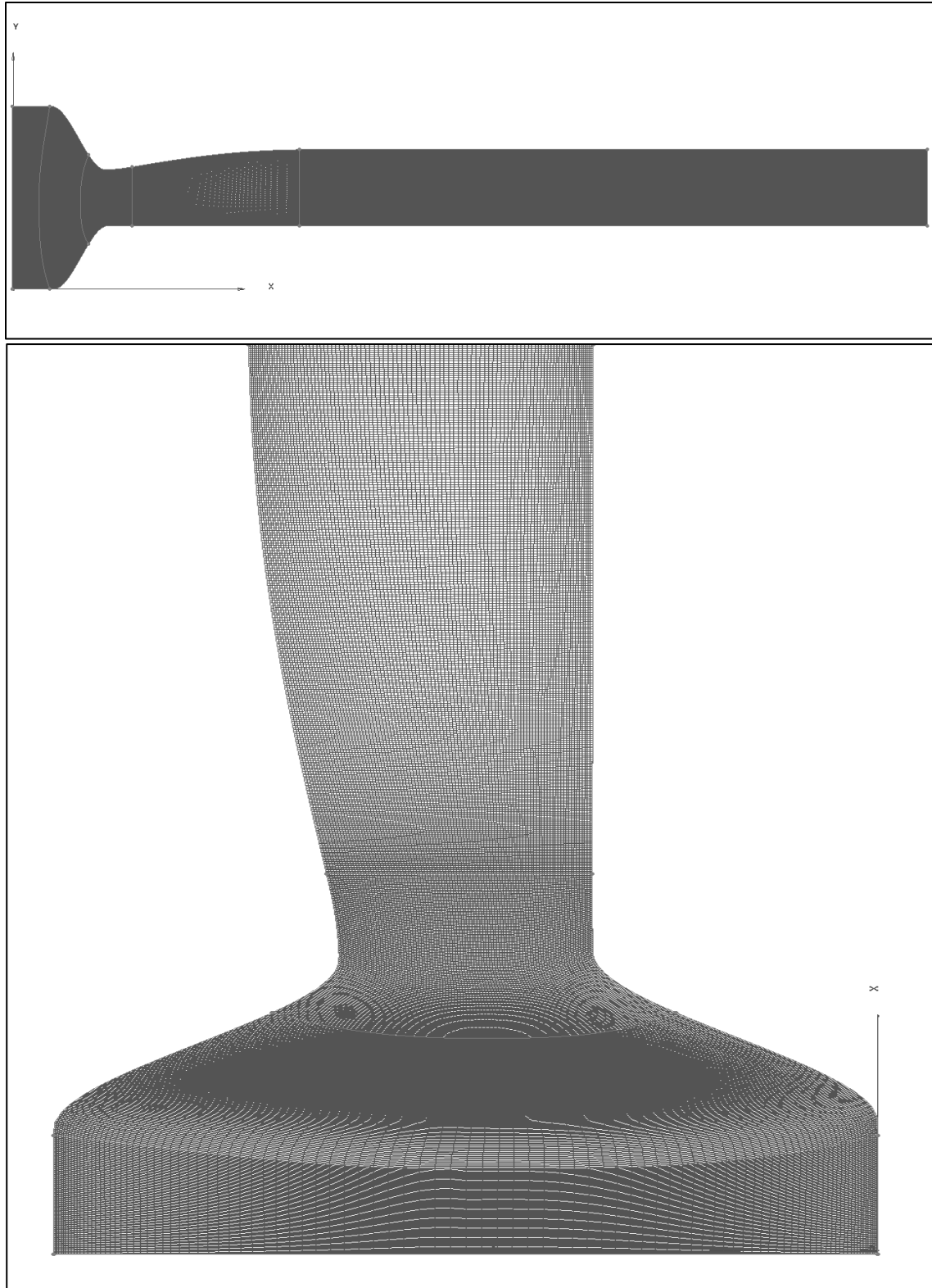
Figure 8. Nozzle/isolator grid: (top) overview, (bottom) nozzle close up
