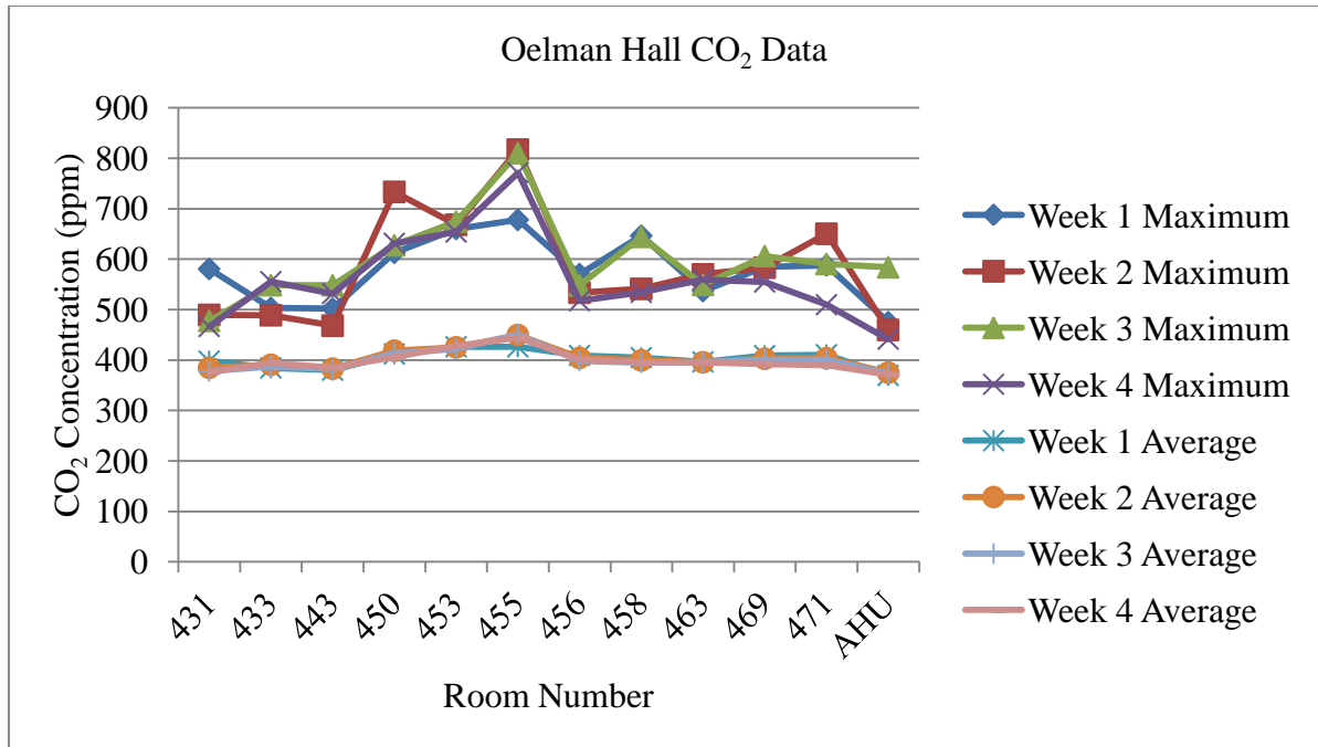
Figure 19. Oelman Hall Maximum and Average CO 2 Concentrations
