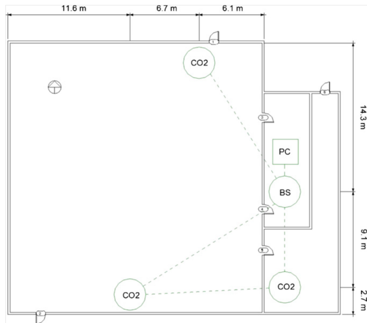
Figure 2. Gymnasium Floor Plan and Sensor Layout (Ng et al., 2011)
