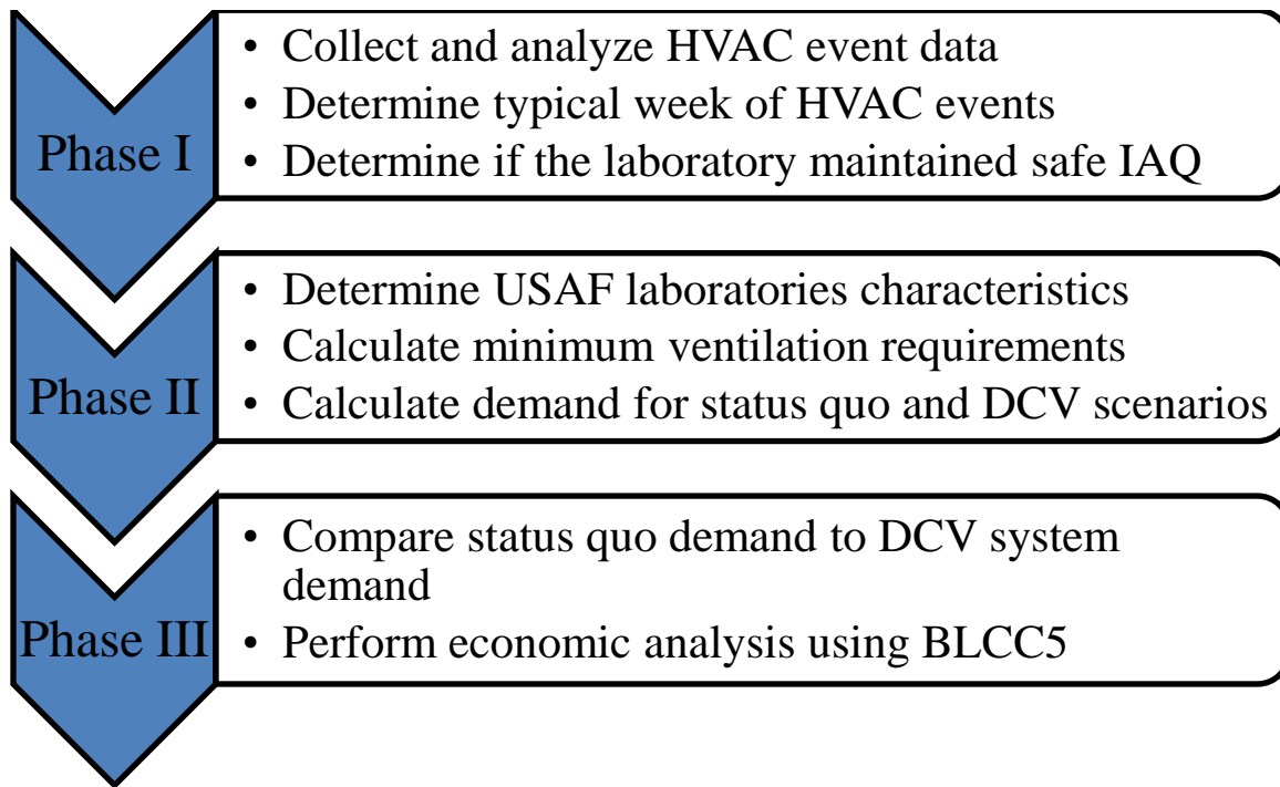
Figure 9. Methodology Process
