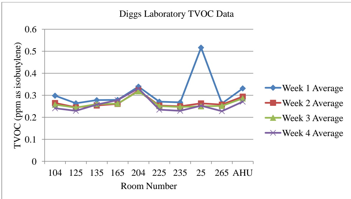
Figure 24. Diggs Laboratory Average TVOC Concentrations
