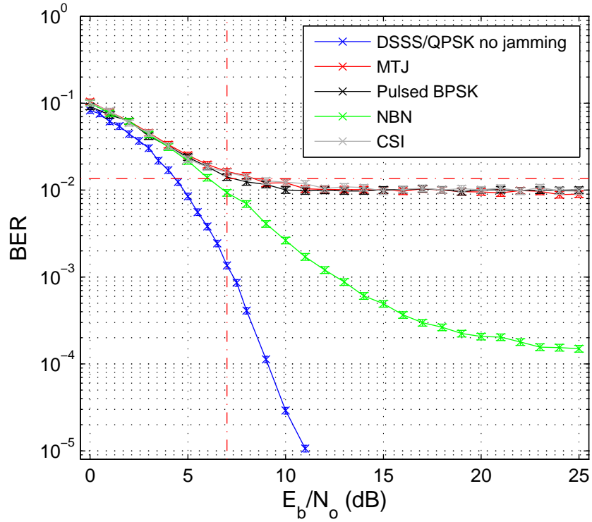
Figure 4.11: BER performance for the optimized jammers at JS R_{RF}=3.1 dB.
