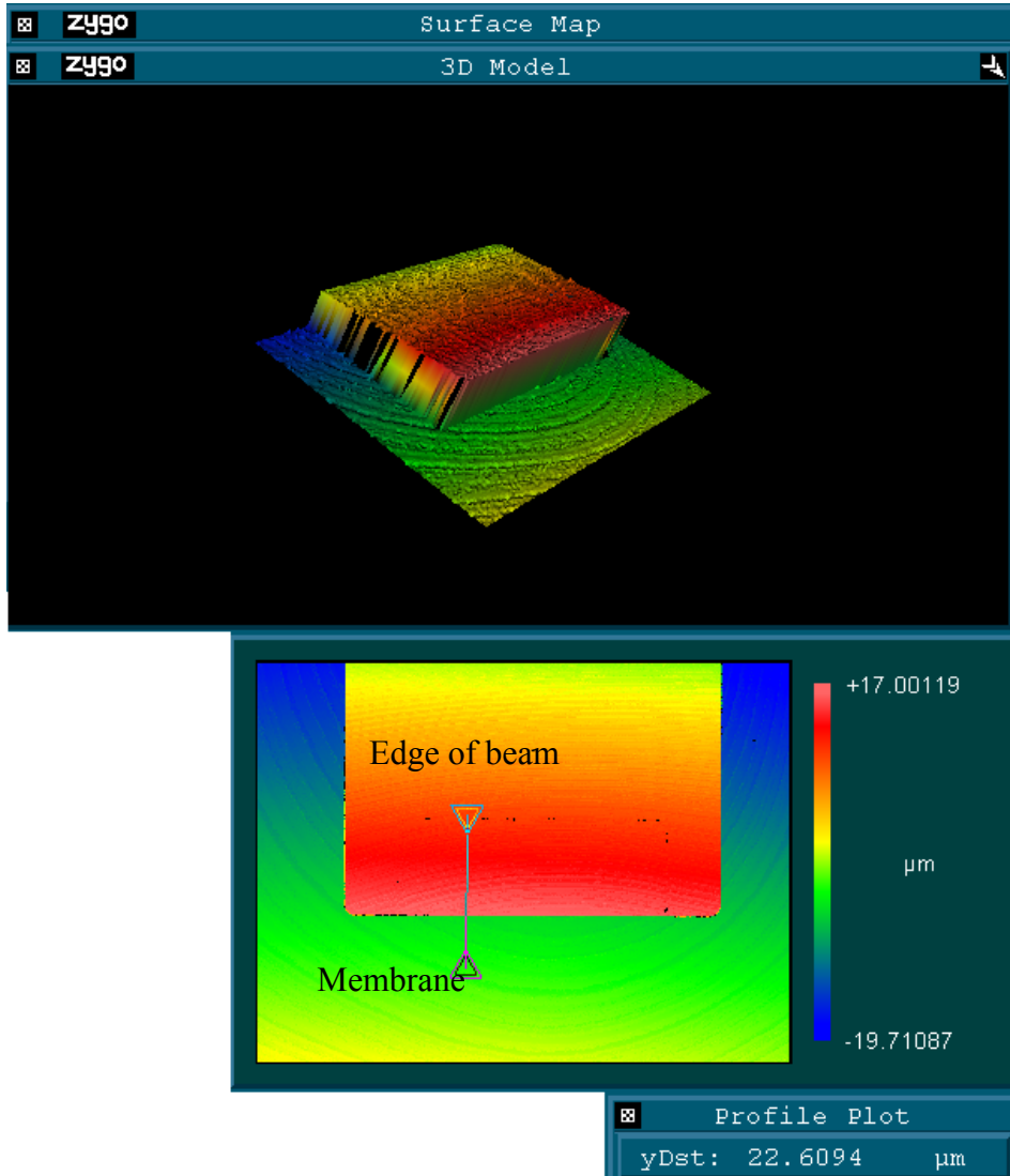
Figure 32 (a). Surface map of cantilever as shown by Zygo TM white light interferometer. The resting curvature of this cantilever beam is 22.6\ \mu\text{m} out of plane measured from the tip to the membrane directly across from it.
