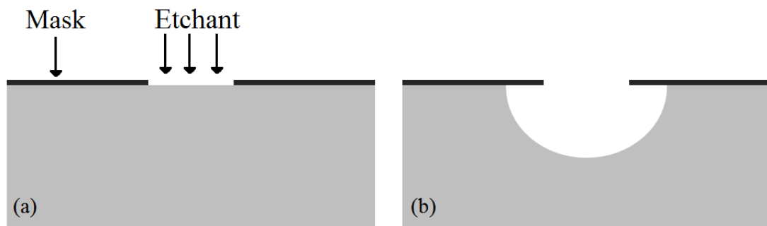
Figure 3. Isotropic etching profile. A mask is applied to the surface of the substrate in (a) and as the etchant reacts with the exposed substrate, it etches equally in all directions. This results in the undercutting of the masking material shown in (b).
