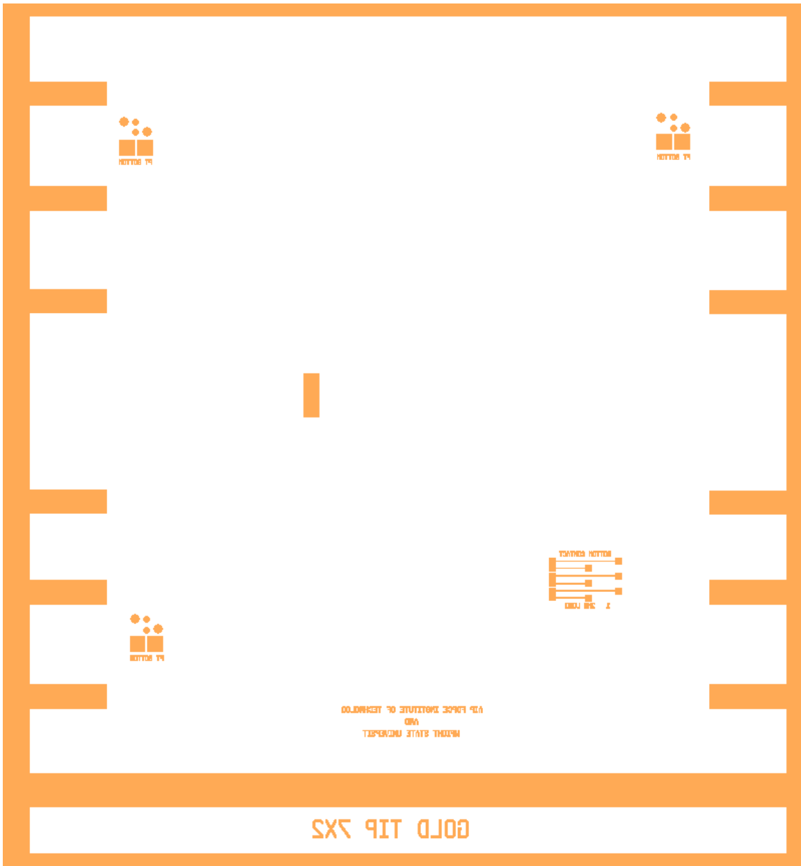
Figure 46. Zoomed view of the gold (Au) spot mask for a 7x2 mm 2 cantilever. The thickness of the beam is up to the user.
