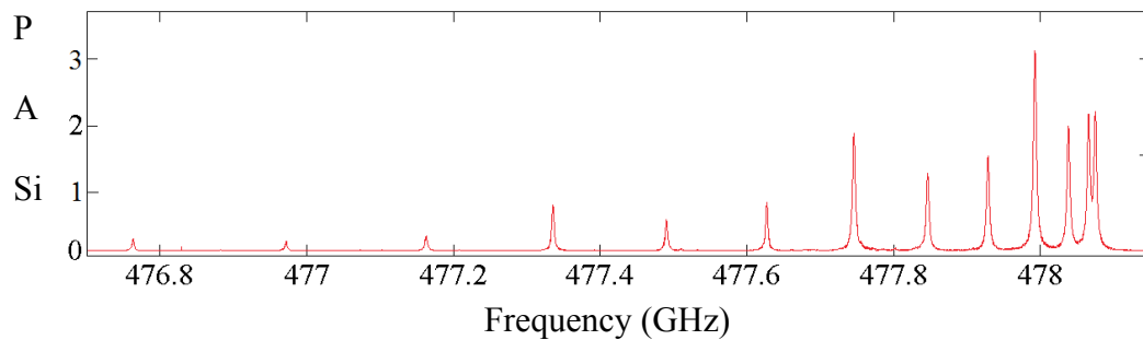
Figure 36. Methyl cyanide spectra of 7\times 2\times 0.01\ \text{mm} cantilever beam taken at 15 mTorr along a \sim 1.5\ \text{GHz} spectrum. The collection shows strong absorption lines as well as high signal to noise (SNR) ratios.
