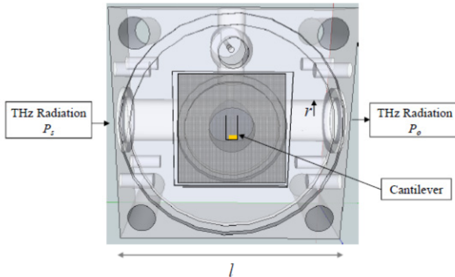
Figure 16. Schematic of back of photoacoustic test chamber [25]. Test chamber is 2 \times 2 \times 2 in 3 and machined from stainless steel. The absorption cell has a radius r = 0.197 in and is sealed at either end with Teflon windows. The cantilever sits between the two halves of the cell and is measured optically with a laser through a window in the front half of the cell.
