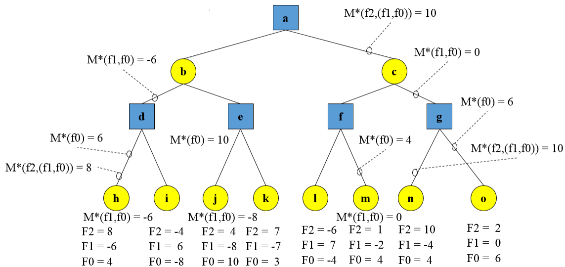
Figure 5: Game tree recursive search of M^* with M^*(a, 3, f_2(f_1, f_0)) [6].
