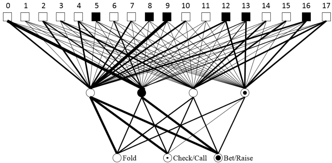
Figure 6: A neural network predicting on opponent’s future action [10].
