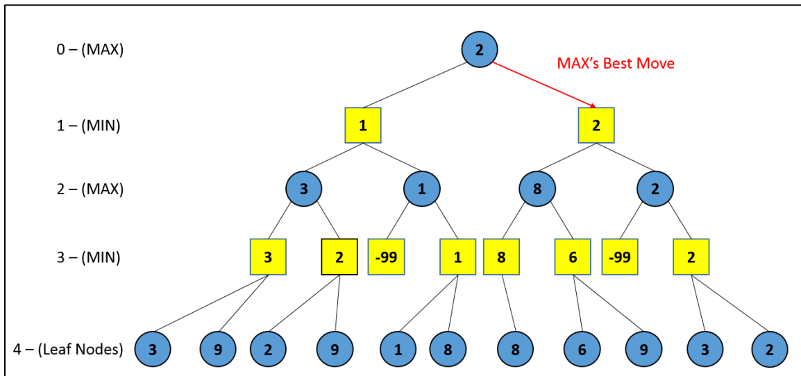
Figure 3: MiniMax game tree.
