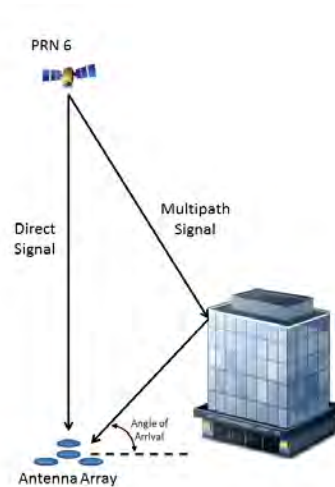
Figure 20. Multipath Diagram
