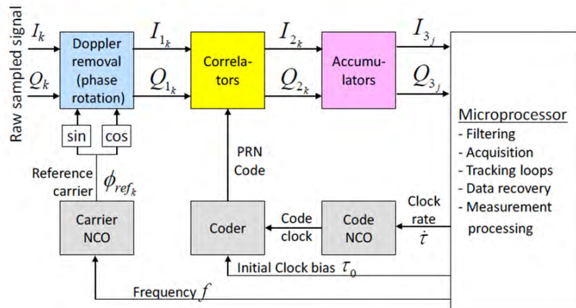
Figure 1. GPS Receiver Algorithm (Figure provided by [10])
