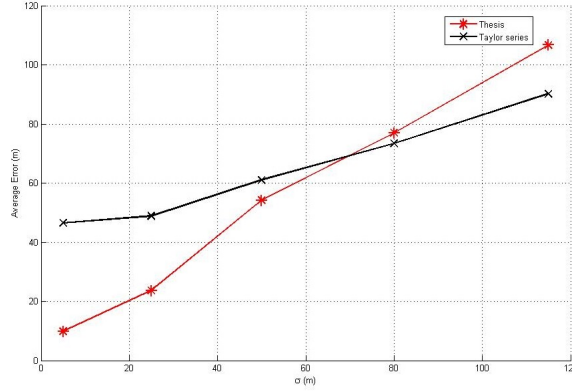
Figure 4.13: For each \sigma_N value, the simulation was run fifty times, and the average error from both methods is plotted. The red stars delineate the error values for this thesis method, and the black X's delineate the error values for the Taylor series method.
