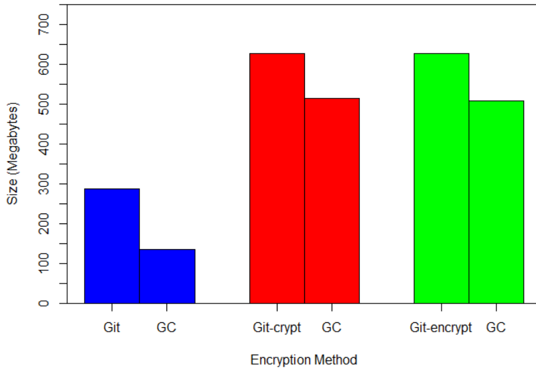
Linux Size After Initial Add (GC Comparison)
