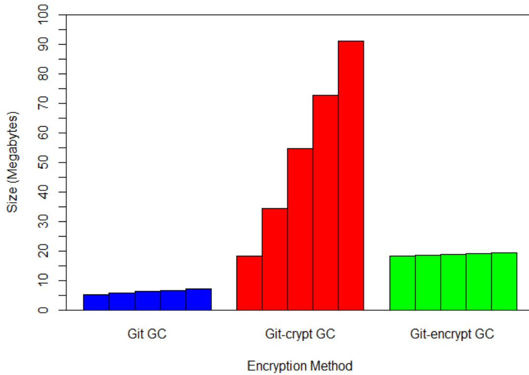
Figure 25. Phase One, Experiment III: Git Program
