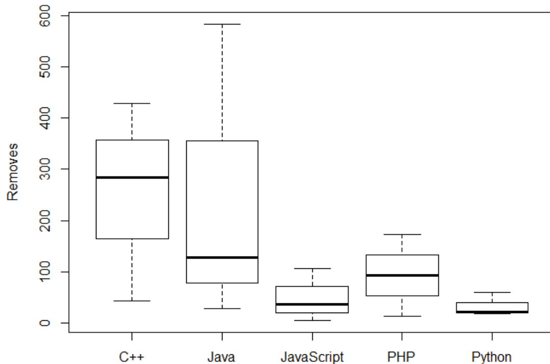
Trending Repository Remove Ave Data
