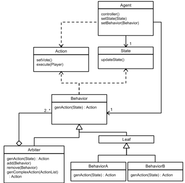
Fig. 9. A UML diagram of the OpenEagles implementation of the Unified Behavior Framework (UBF).
