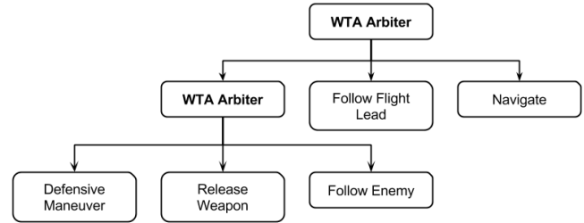
Fig. 10. The UBF behavior tree for the sweep mission scenario.
