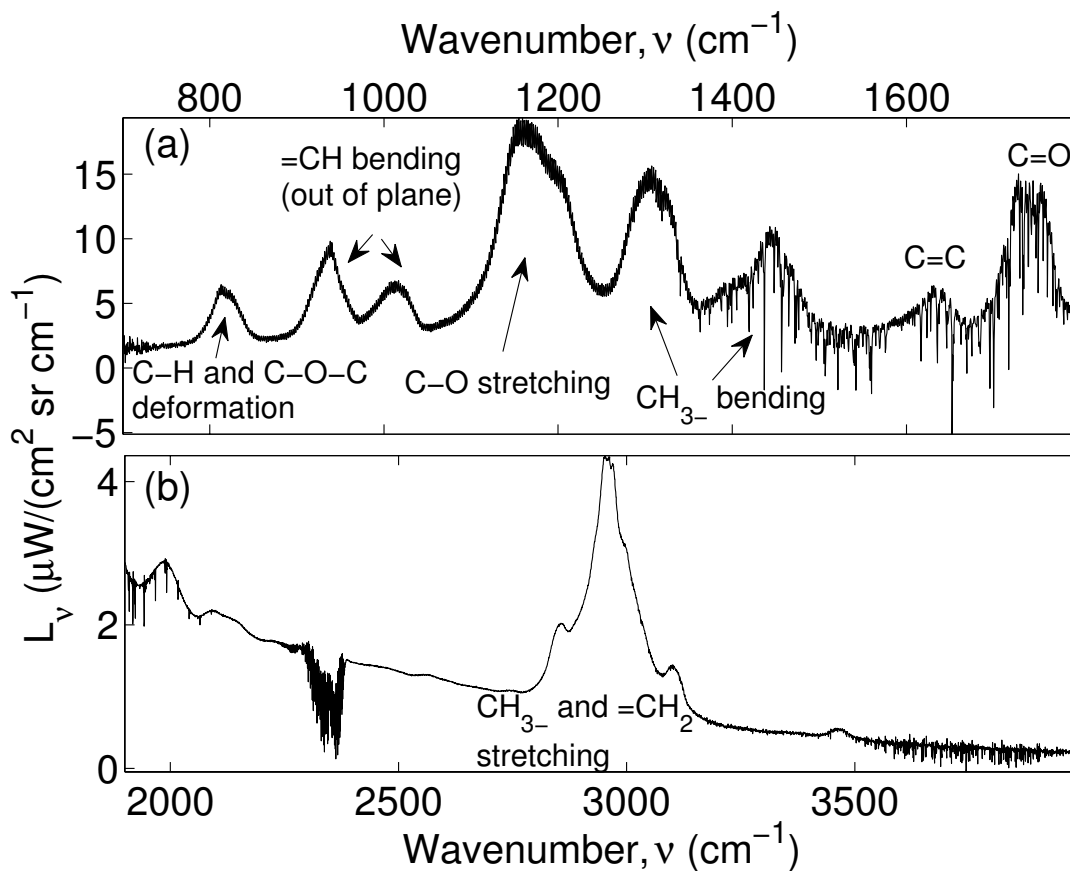
Figure 19. Non-imaging FTIR time averaged spectra for laser irradiated PMMA at 21.7 W/cm 2 showing the spectral radiance ( L_\nu ) of MMA in the (a) LWIR and (b) MWIR.
