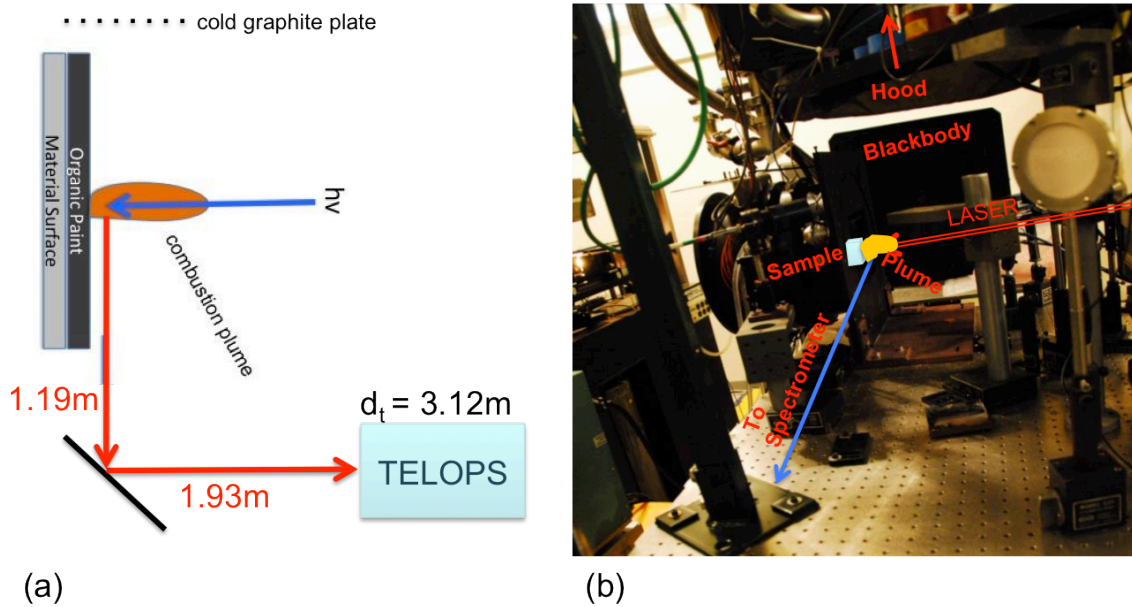
Figure 50. (a) Top view for schematic diagram of the experiment set-up with the IFTS perpendicular to the combustion plume for the laser irradiation event. (b) Photo of the actual testing set-up with the sample normal to the laser energy and a cold blackbody plate positioned at the instrument FOV perpendicular to the combustion plume.
