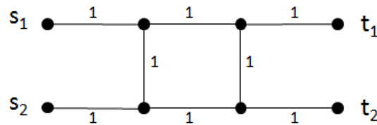
Figure 2.9. Multicommodity Flow Problem d_1 = d_2 = 1 [5]
