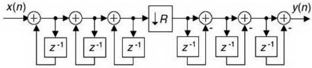
Figure 2.6: Example CIC Design with n_s = 3 Stages [15]. The \oplus Symbols Denote Modulo-2 Addition, Z^{-1} Denotes a Delay by One Clock Cycle, and \downarrow R Denotes Down-Sampling (Decimation).
