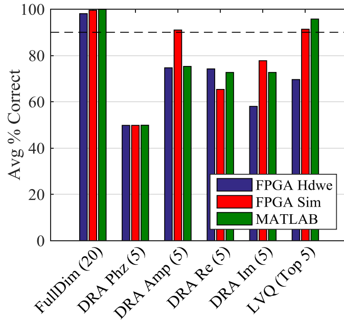
Figure 4.7: Comparison of Qualitative (Phz, Amp, Re, Im) and Quantitative (LVQ) DRA Performance with Full Dimensional Performance using \vec{F}_M , \vec{F}_S , and \vec{F}_H Generated Fingerprints. The Number of Features per Feature Set is Indicated in Parenthesis.
