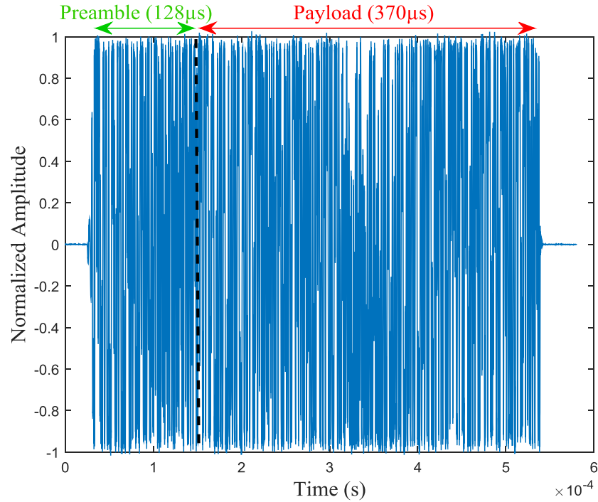
Figure 4.2: Representative X310 SDR Collected ZigBee Burst Amplitude Response Showing Preamble and Payload Regions.
