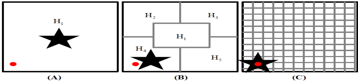
Figure 18. An example of the division of a pixel into sub-pixel locations for varying M . (A) BHT with M=2 (B) MHT with M=6 (C) MTH with M=122 .
