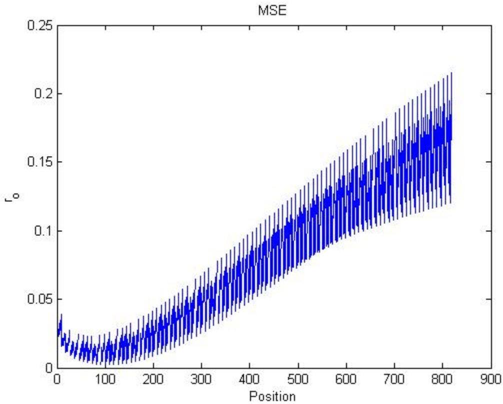
Figure 40. Obtaining L_0 value for AFIT telescope experiment via MSE technique.
