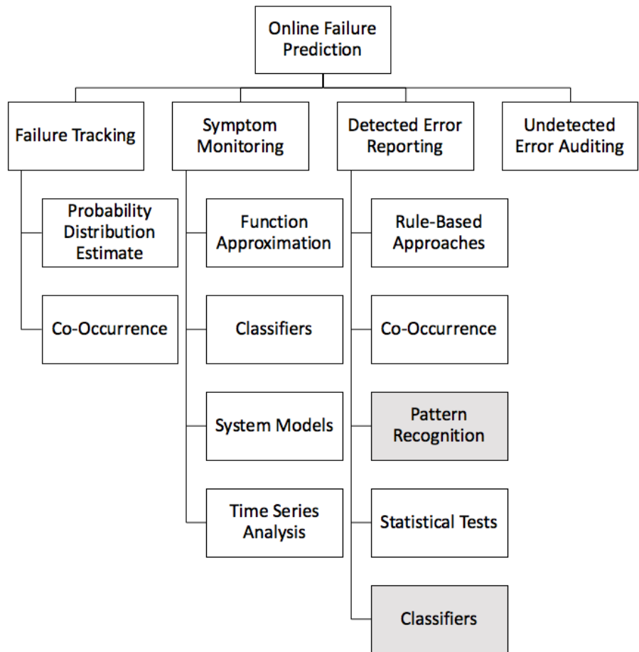
Figure 4. Taxonomy of approaches to online failure prediction [1]. The two categories into which this research falls are highlighted.
