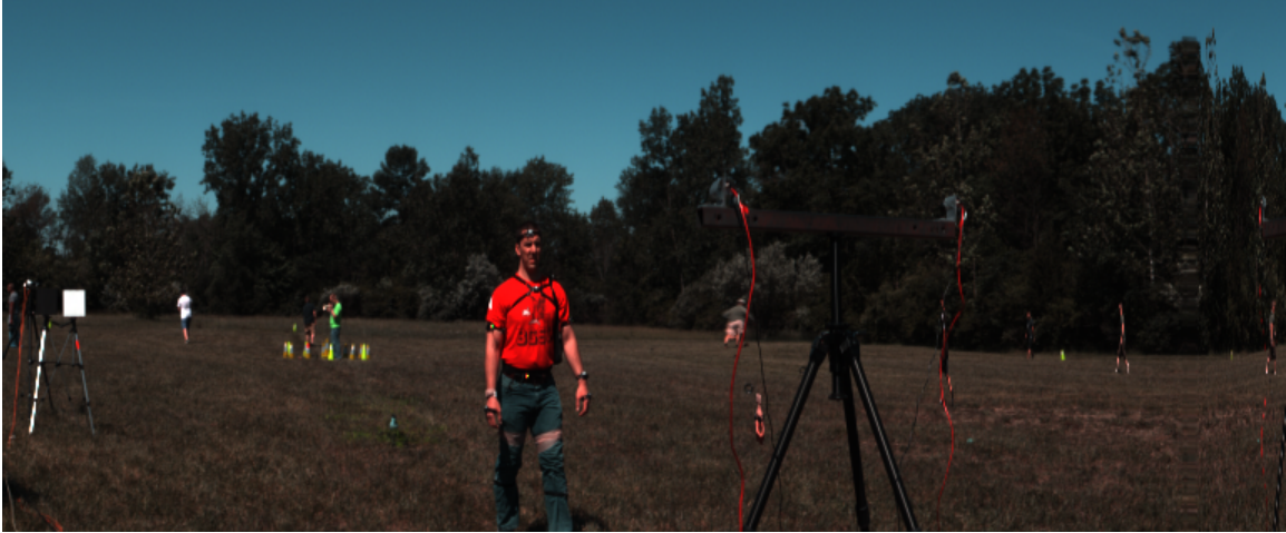
Figure 4.2. A color representation of the hyperspectral image used for detection in this thesis.
