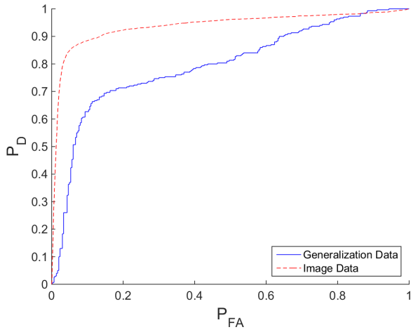
(c) [5 4 2 1], AUC_{GEN} = 0.797 , AUC_{IM} = 0.938
