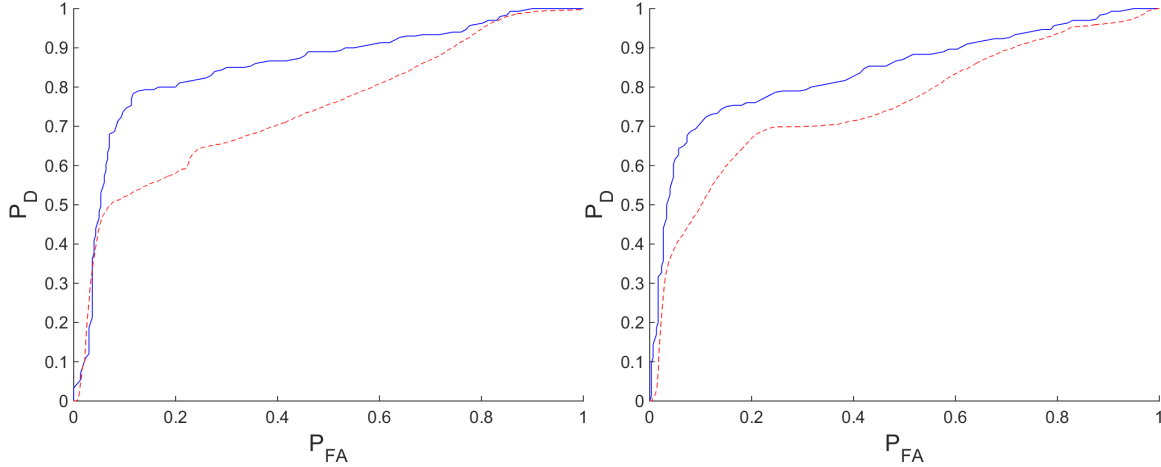
(a) [4 6 4 1], AUC_{GEN} = 0.852 , AUC_{IM} = 0.743
