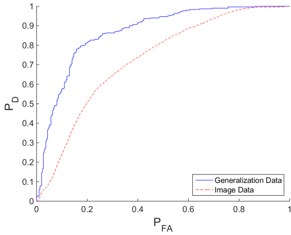
(c) [5 6 2 1 1], AUC_{GEN} = 0.866 , AUC_{IM} = 0.726
