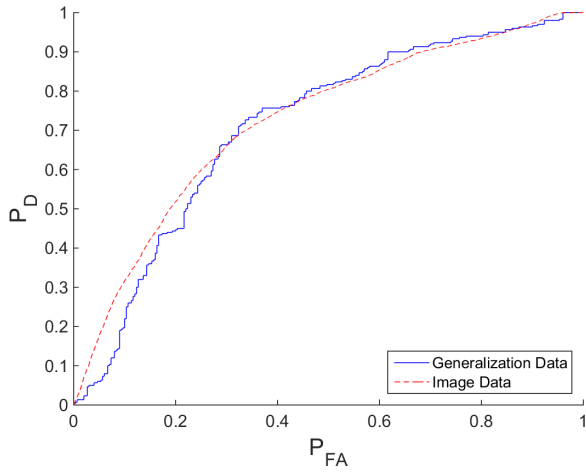
(c) [1 1 3 3 1], AUC_{GEN} = 0.712 , AUC_{IM} = 0.724
