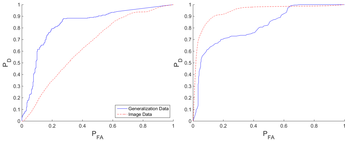
(c) SFS Noiseless feature set, [6 1]
