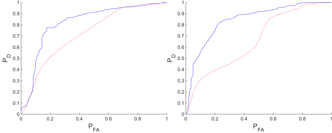
(a) [5 5 2 1], AUC_{GEN} = 0.819 , AUC_{IM} = 0.723
