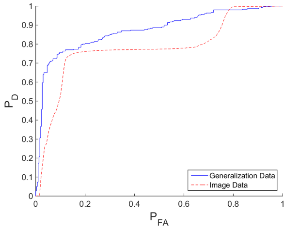
(c) [4 5 6 1], AUC_{GEN} = 0.872 , AUC_{IM} = 0.778
