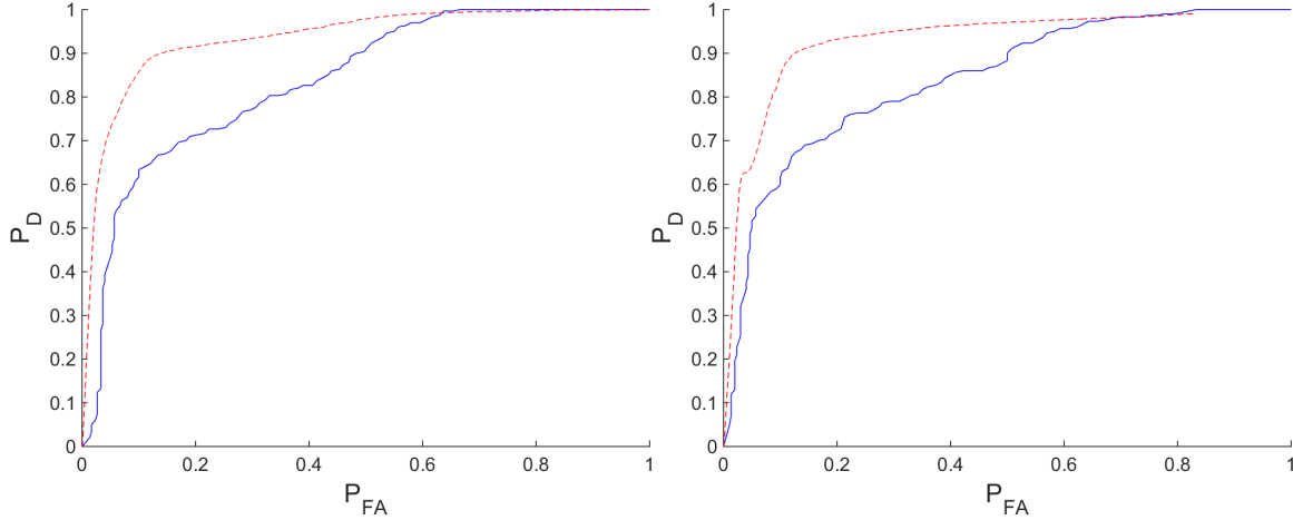
(a) [5 4 1 1], AUC_{GEN} = 0.838 , AUC_{IM} = 0.935
