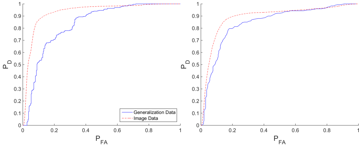
(c) SFS Noiseless feature set, [6]
