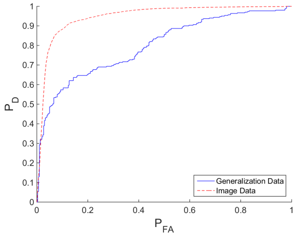
(c) [4 6 5 1], AUC_{GEN} = 0.799 , AUC_{IM} = 0.947
