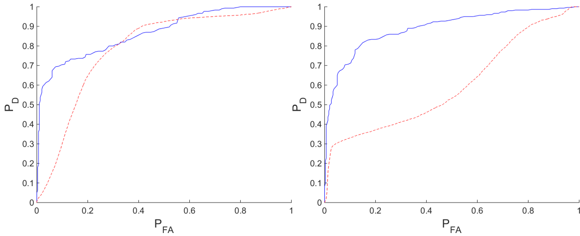
(a) FCBF Noiseless feature set, [5 3]
