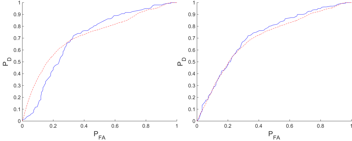
(a) [1 3 3 1], AUC_{GEN} = 0.709 , AUC_{IM} = 0.723
