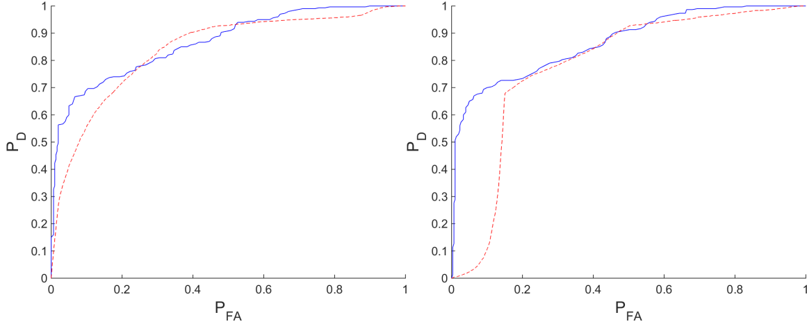
(a) [2 4 4 1], AUC_{GEN} = 0.868 , AUC_{IM} = 0.838
