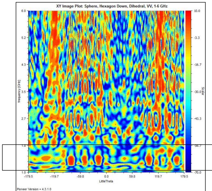
Figure 35: Sphere w/Dihedral, Hexagon Down, VV
