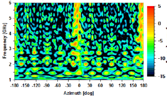
UNCLASSIFIED Sphere with Flat Plate, Pentagon Down, VV
