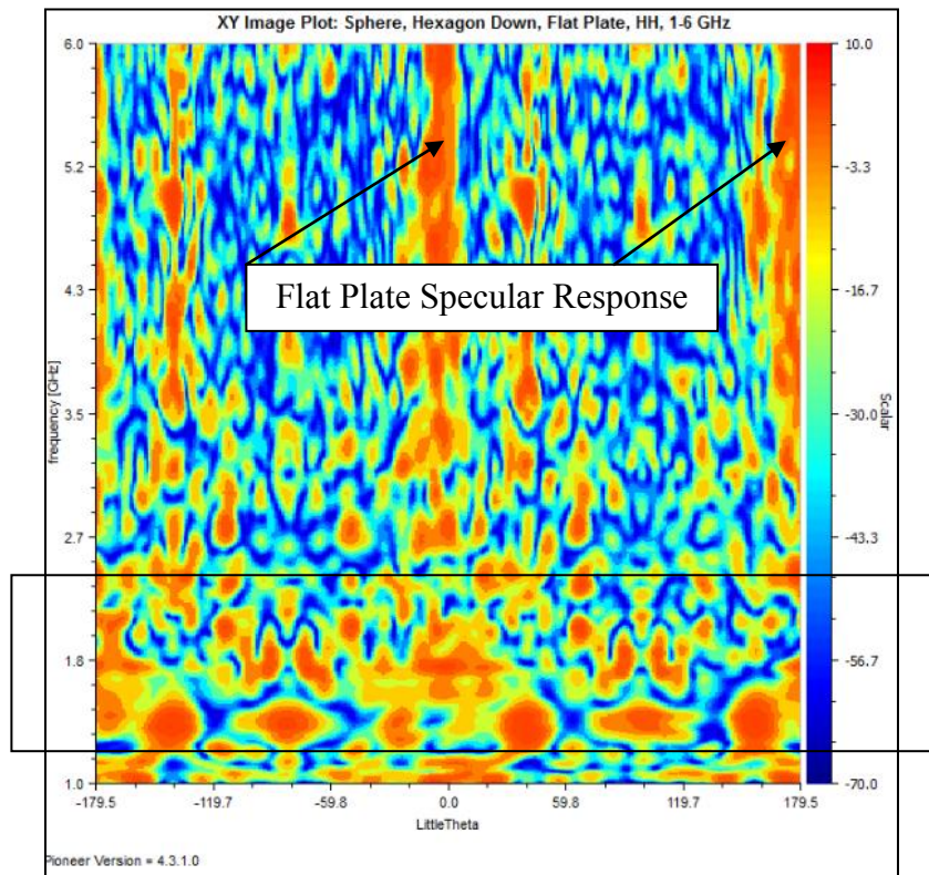
Figure 29: Sphere w/Flat Plate, Hexagon Down, HH
