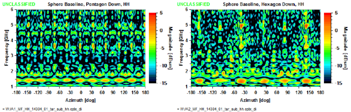
Figure C2: GFP Sphere Baseline Results, HH
