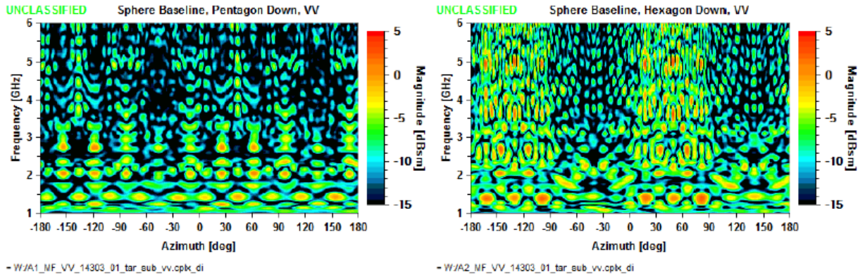
Figure C4: GFP Sphere Baseline Results, VV
