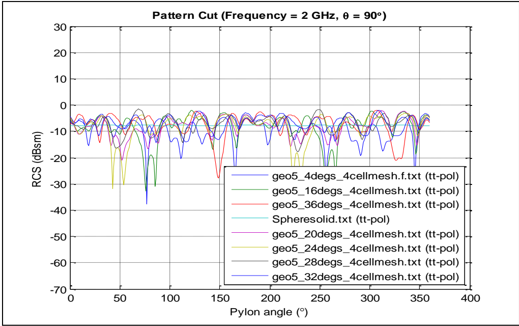
Figure 45: RCS Magnitude vs. Pitch Angle
