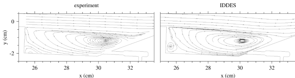
Figure 8. Streamlines calculated from mean velocity for both the experiments and Peterson’s simulations.[6]
