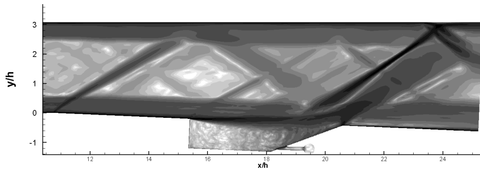
(b) Time-Averaged
