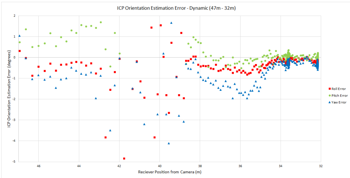
Figure 31. Orientation Estimation Error for ICP of the Dynamic Reference Model with Collision Detection (Region C)
