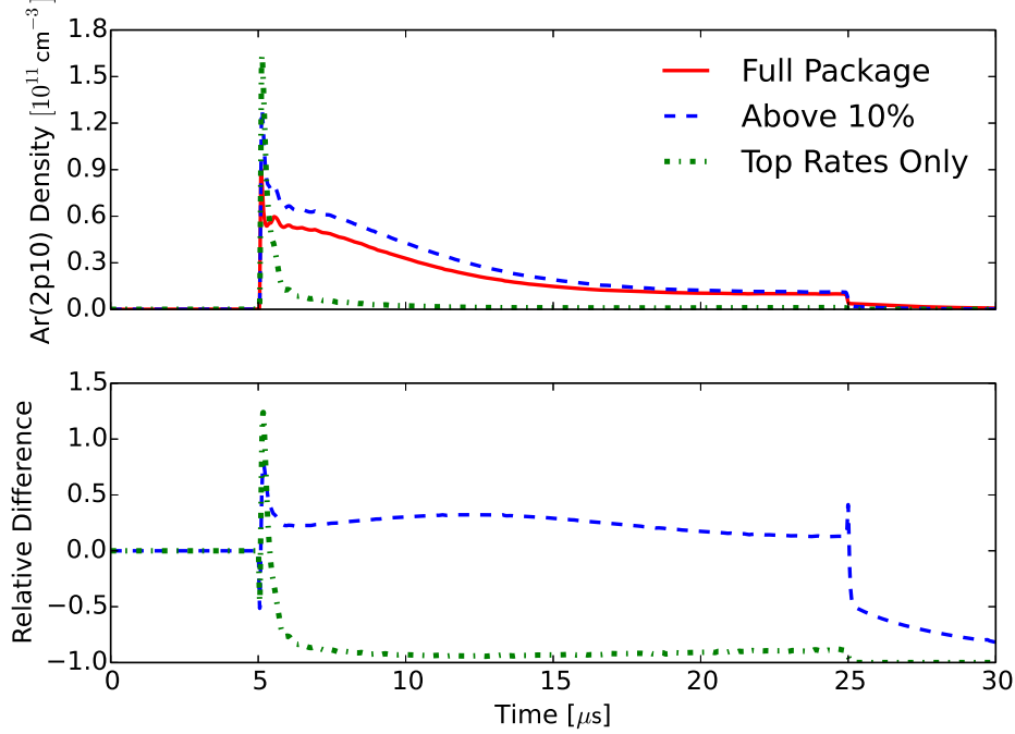
Figure 22. Simulated Ar(2p_{10}) densities for a 20 \mu\text{s} pulse, using the full reaction rate package and two reduced packages, along with the relative difference between the reduced rate packages compared to the full rate package.
