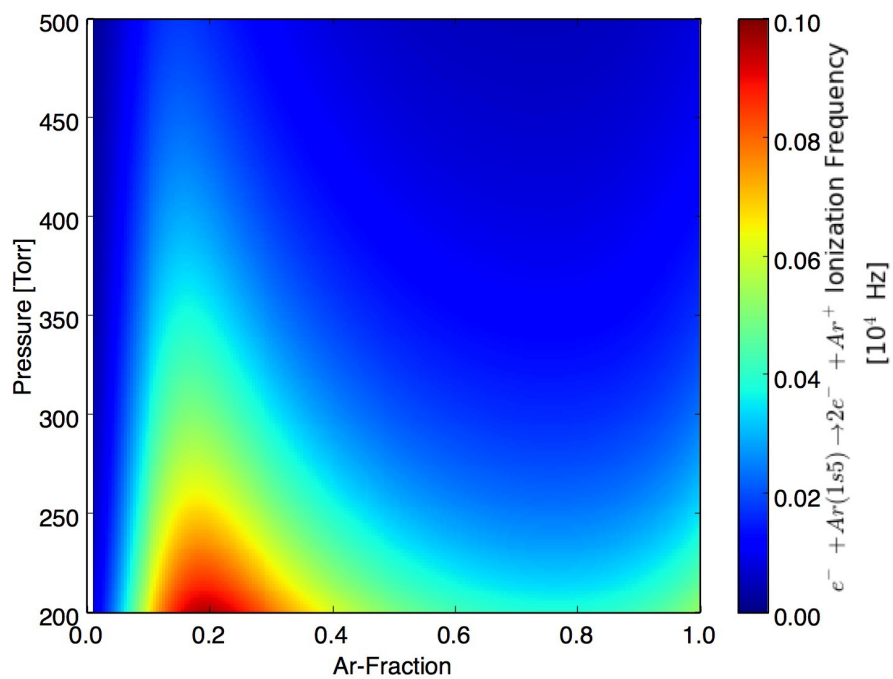
Figure 109. Ionization frequency of Ar(1s_5) + e^- \rightarrow Ar^+ + 2e^- as a function of Ar-fraction and pressure.
