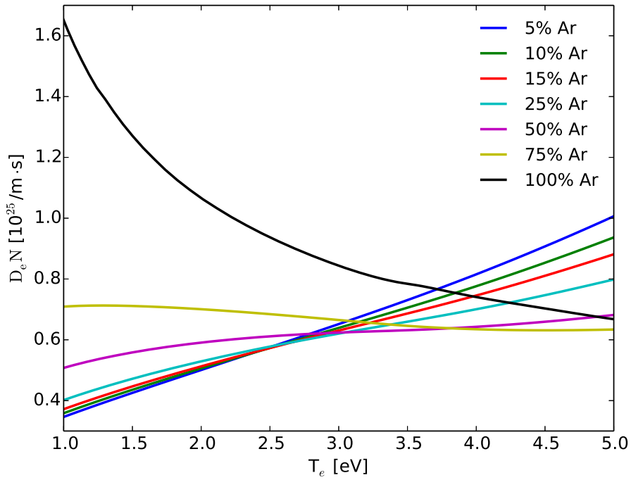
Figure 38. Electron diffusion coefficients for varying Ar-He mixtures, as calculated by BOLSIG+.
