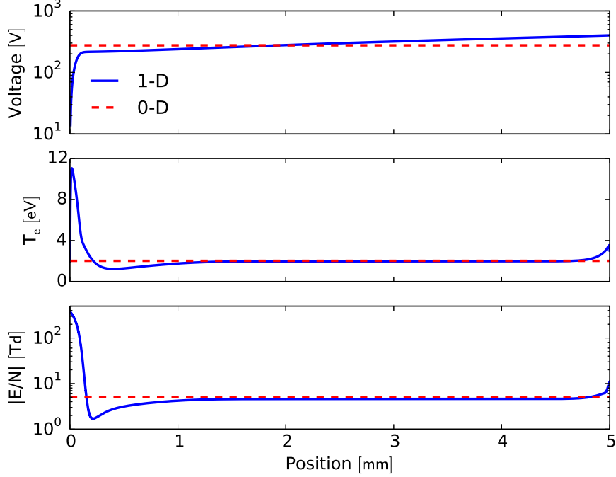
Figure 26. Spatial profile of voltage, T_e , and E/N magnitude at the end of the 20 \mu\text{s} pulse.
