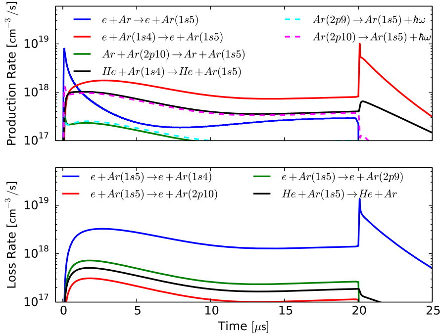
Figure 18. Positive column Ar(1s_5) production and loss rates over time. After pulse termination, the decrease in T_e causes a collapse in the EEDF towards lower energies, which increases Ar(1s_5) + e^- \leftrightarrow Ar(1s_4) + e^- rates.
