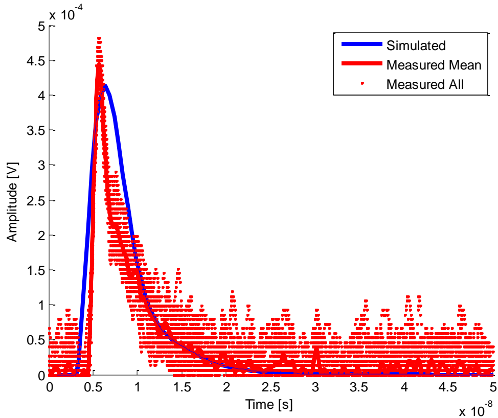
Fig. 41. The simulated waveform of a single pixel firing event is shown compared to the measured response of 25 of single pixel waveforms (and their mean) from MPPC#1 at 73 V bias.
