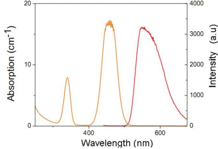
Fig. 5. The absorption or excitation (orange) and emission (red) properties of single crystal fiber YAG:Ce is shown. The overlap of emission and absorption curves indicates self-absorption. The data shown is adapted from [21].
