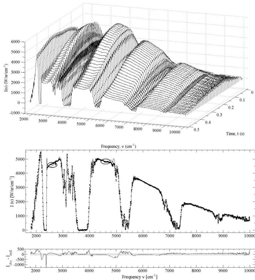
Figure 19. (a) Temporally-resolved spectra for event E9, and (b) the FTS observed spectral intensity (•) of event E9 at 0.28 s after detonation. Two spectral regions: 2500–2700 and 4500–4700 \text{cm}^{-1} , of continuum radiation are indicated for the two-color temperature determination. A fit of the observed spectra (—) to the radiative transfer model of Eq. (15) yields fit residuals of \sim 3.7\% , except in the vicinity of the \text{CO}_2 4.3 \mu\text{m} band.
