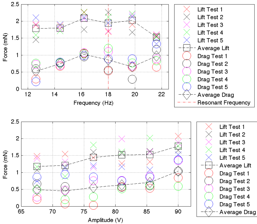
Figure 57: Wing Design 3 Aerodynamic Results
