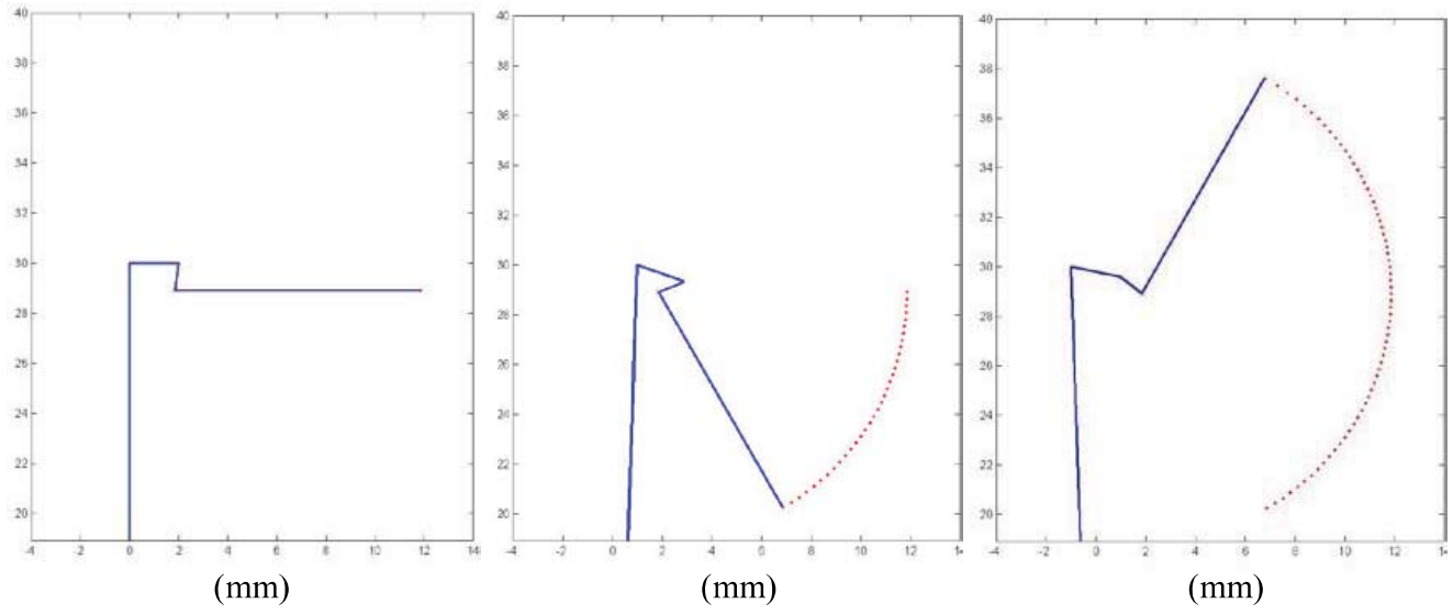
Figure 33: Flapping Actuator Deflection Simulation [1]
