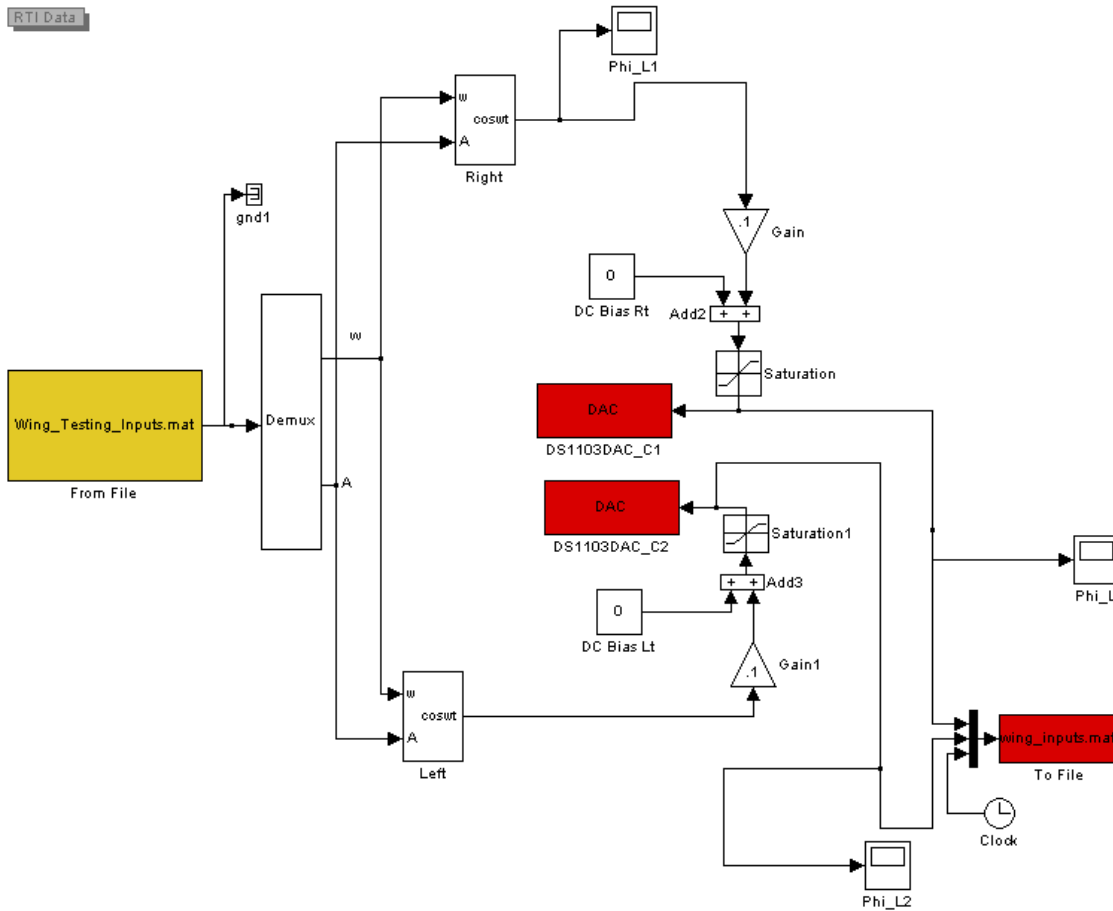
Figure 36: Simulink Model
