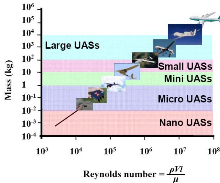
Figure 5. Typical Reynolds number regimes for various aircraft
