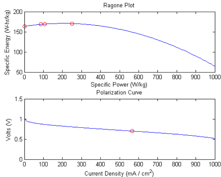
Figure 17. Ragone plot and polarization curve
