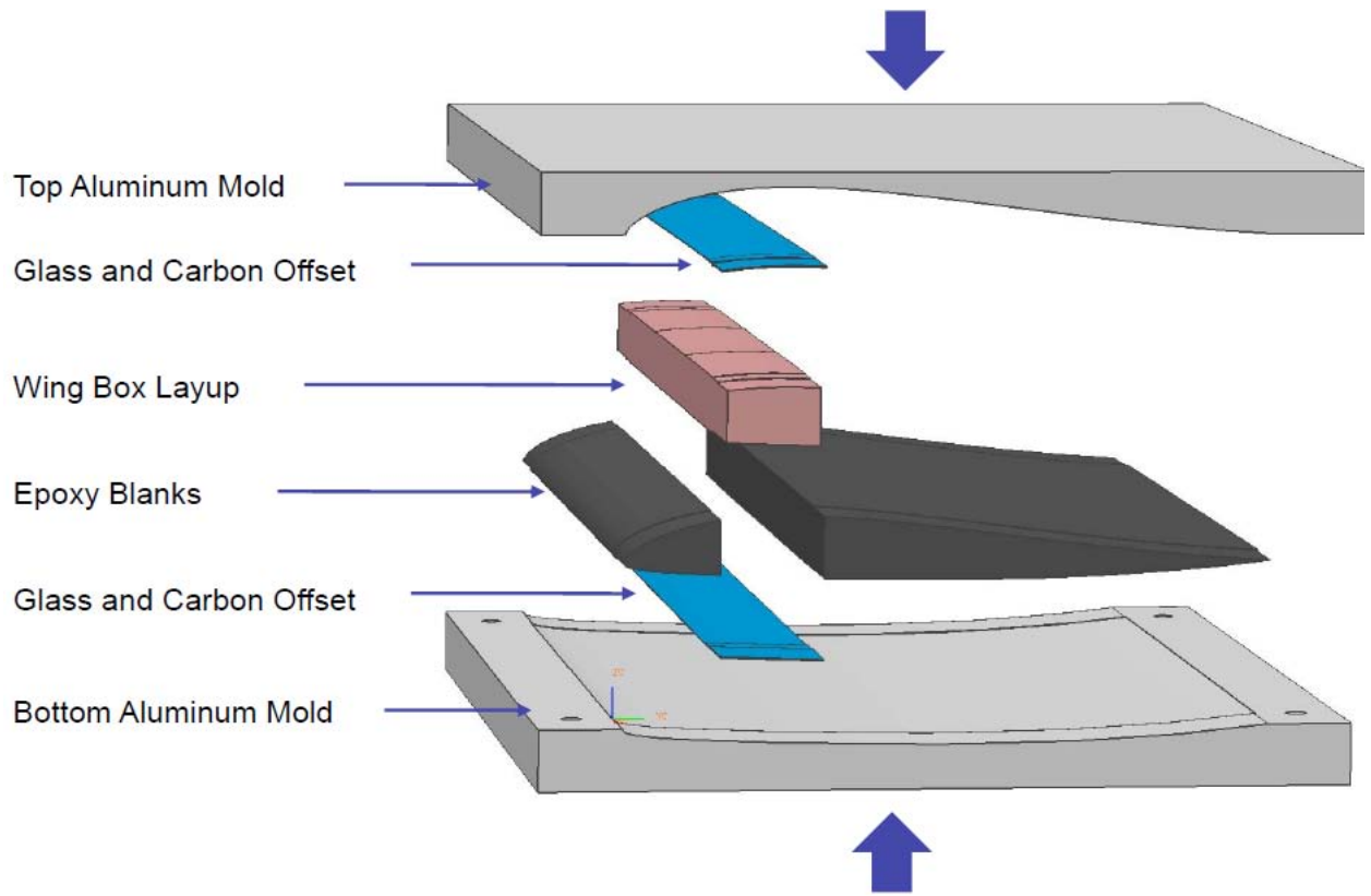
Figure 35. Box Curing Mold Diagram [5]
