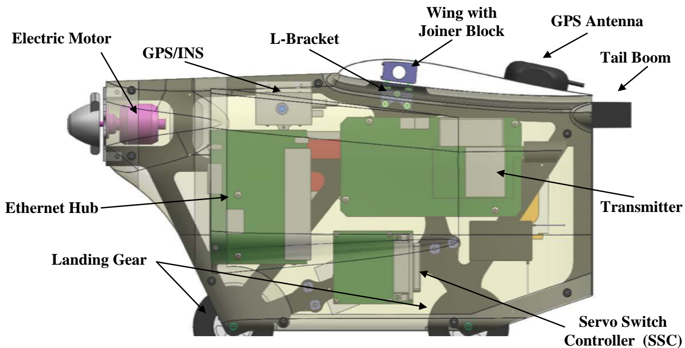
Figure 45. Spine with Internal Components (Right View) [5]
