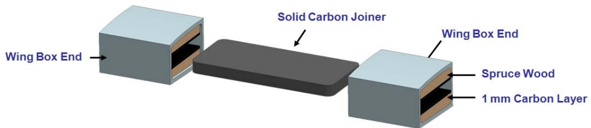
Figure 22. Second Joiner Block Design Iteration [23]
