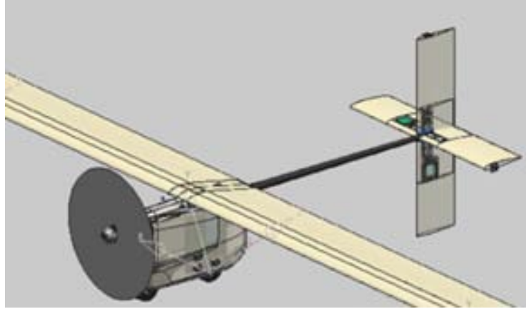
Figure 59. Original X-HALE Center Tail Configuration
