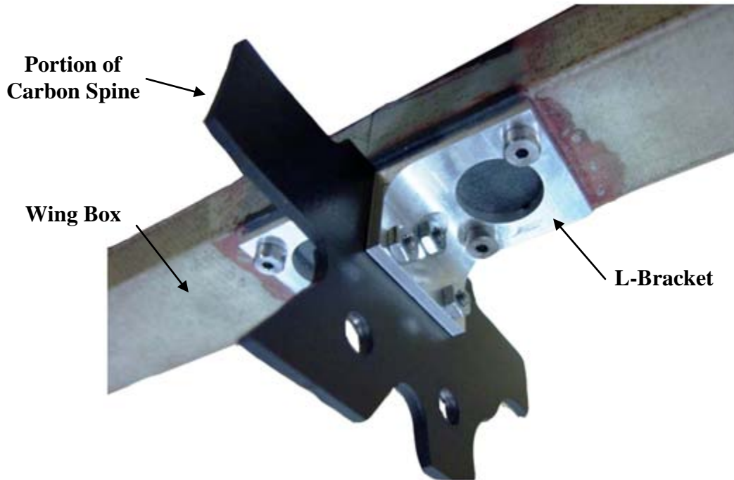
Figure 43. L-Bracket Attachment Sample [5]
