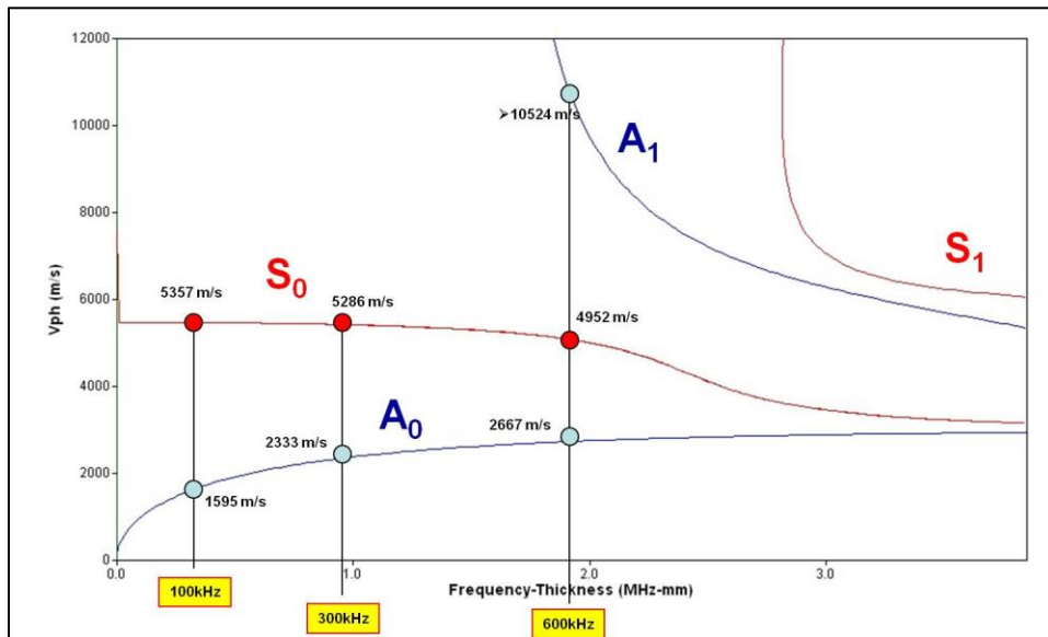
Figure 13: Dispersion Curve for Aluminum using Disperse
