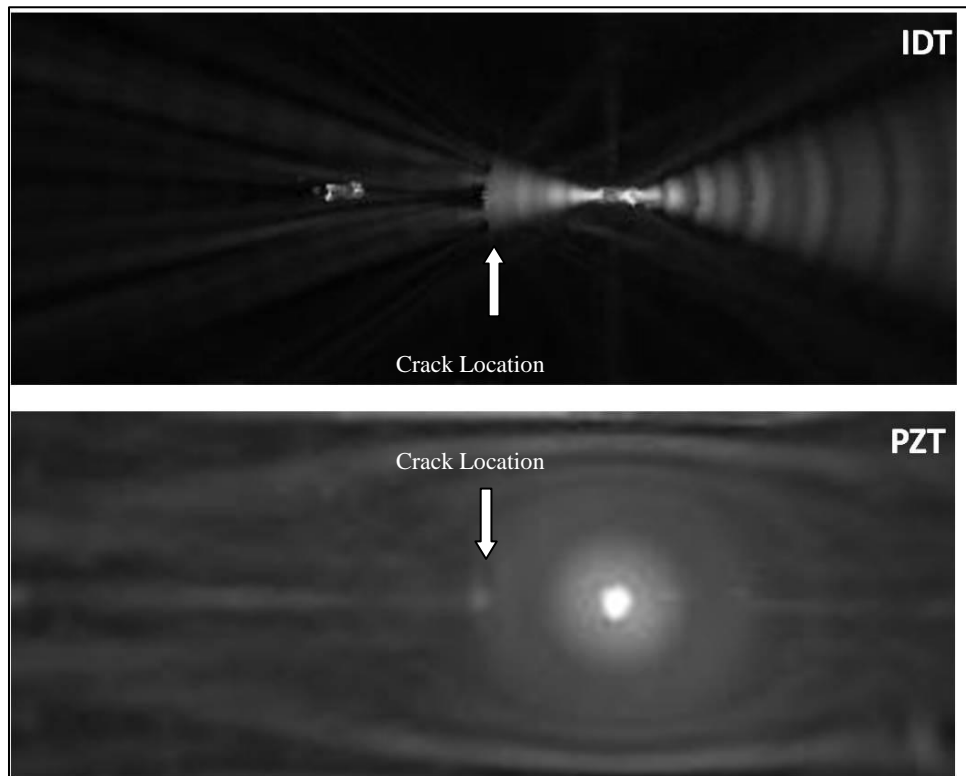
Figure 68 : IDT versus PZT energy over test area
