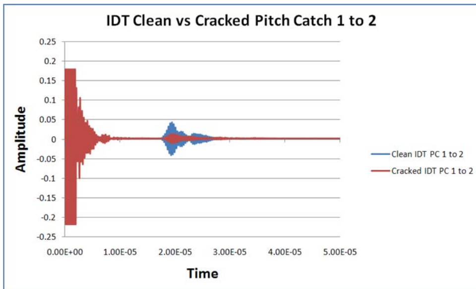
Figure 61 : PZT versus IDT Comparison in Pitch Catch 1 to 2
