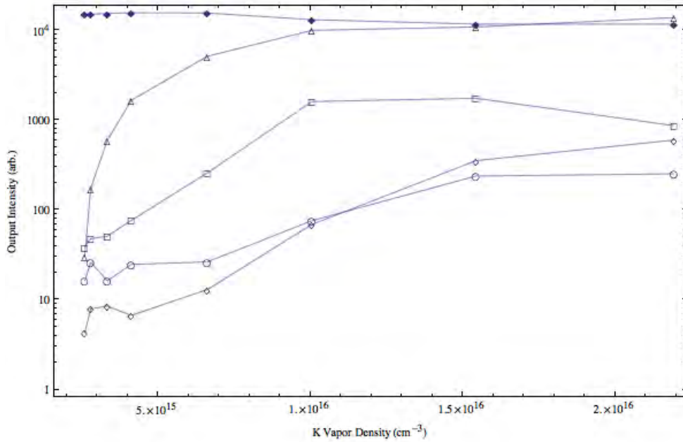
Figure 32. Average output intensity as a function of potassium density for a pump power of 232 mW. Pump ( \blacklozenge ), 1 st anti-Stokes ( \triangle ), 1 st Stokes ( \square ), 2 nd anti-Stokes ( \circ ), 2 nd Stokes ( \diamond )
