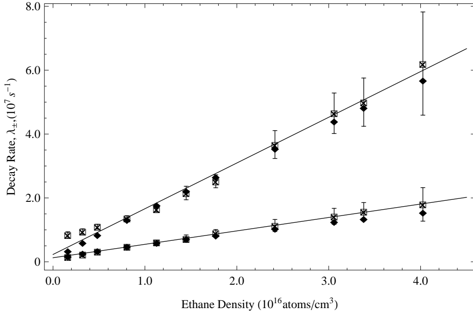
Figure 10. Stern-Volmer plot of experimentally derived rates ( \square ) and calculated rates based on Eq. 22 ( \blacklozenge ) for ethane at 120^\circ\text{C} . The solid line is a least squares linear fit to the experimentally derived rates.
