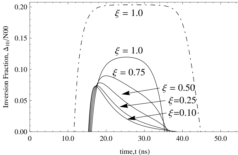
Figure 27. Predicted population inversion for several values of \xi , as a fraction of the initial ground state concentration for an infrared DPAL (- - -) and blue DPAL(—) assuming no stimulated emission. The quenching cross section for the infrared case is 1 \text{ \AA}^2 and 10 \text{ \AA}^2 for the blue case
