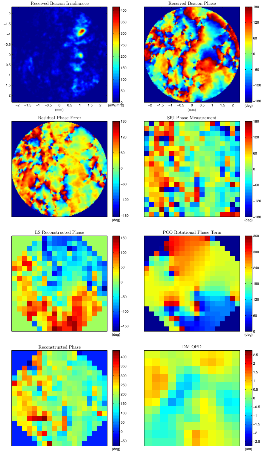
Figure 4.17: AO system state as the higher-order control loop is closing in conditions of \sigma_x^2 = 1 , d/r_0 = 1 , SNR=60. LSPV+4 is the wavefront reconstructor.
