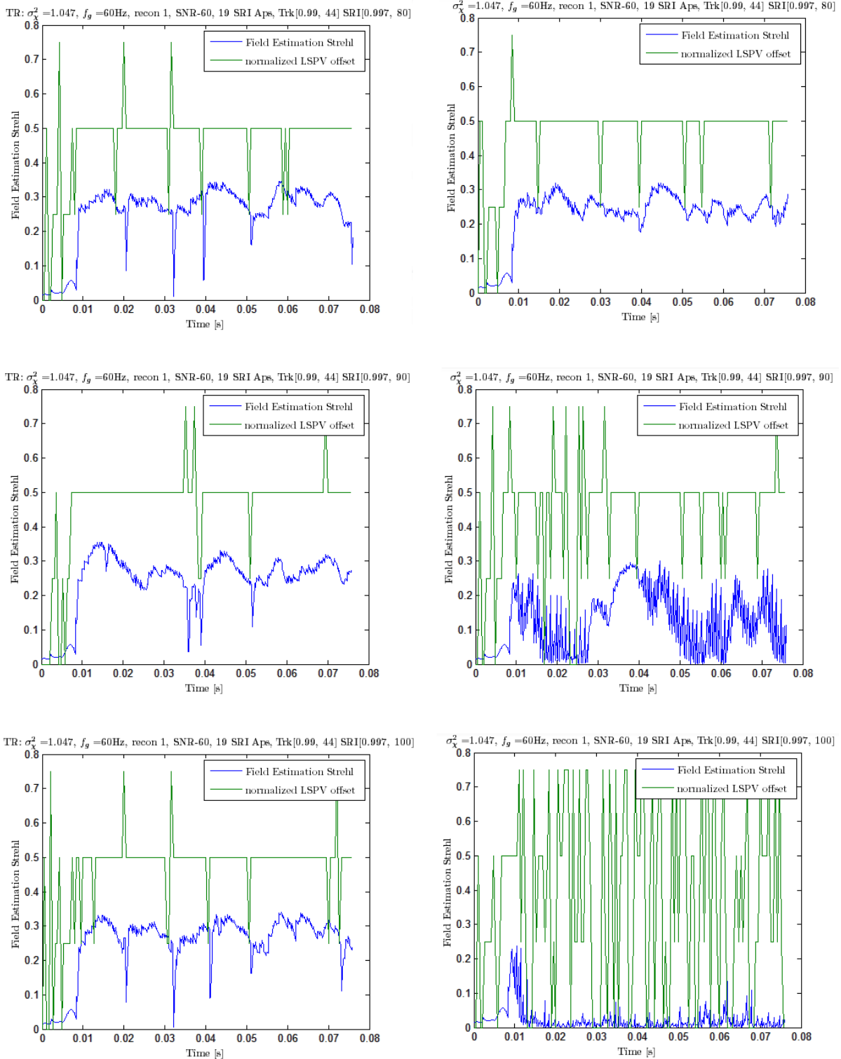
Figure 4.11: Plots of AO performance with tilt decoupled (left column) and tilt coupled (right column) between the two control systems. Each row implements an increasing higher-order control gain.
