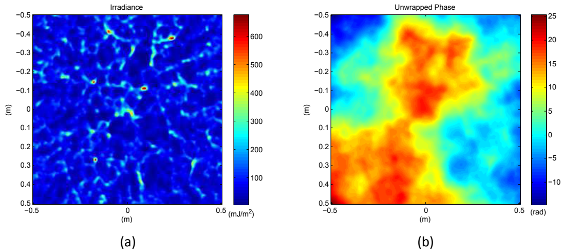
Figure 2.11: Received point source irradiance(a) and phase(b) propagated through weak turbulence.
