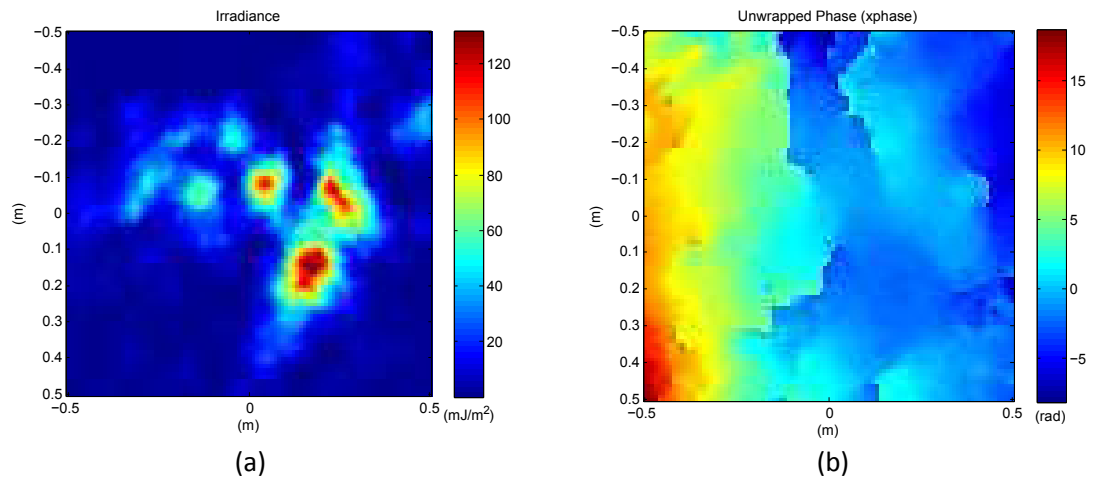
Figure 2.12: Received point source irradiance(a) and phase(b) propagated through strong turbulence.
