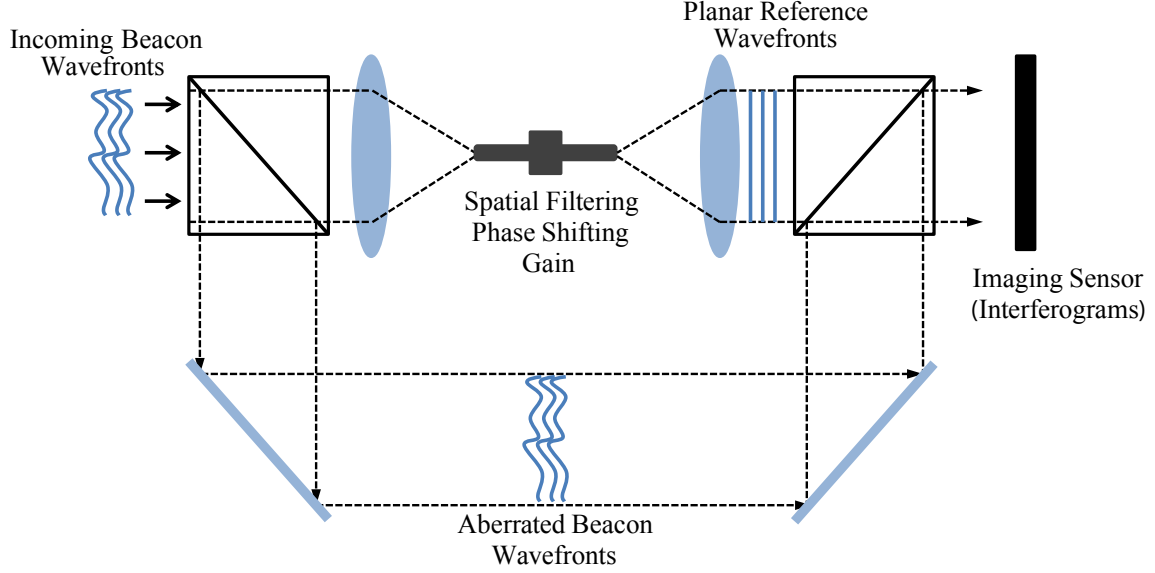
Figure 2.6: The Self-Referencing Interferometer.
