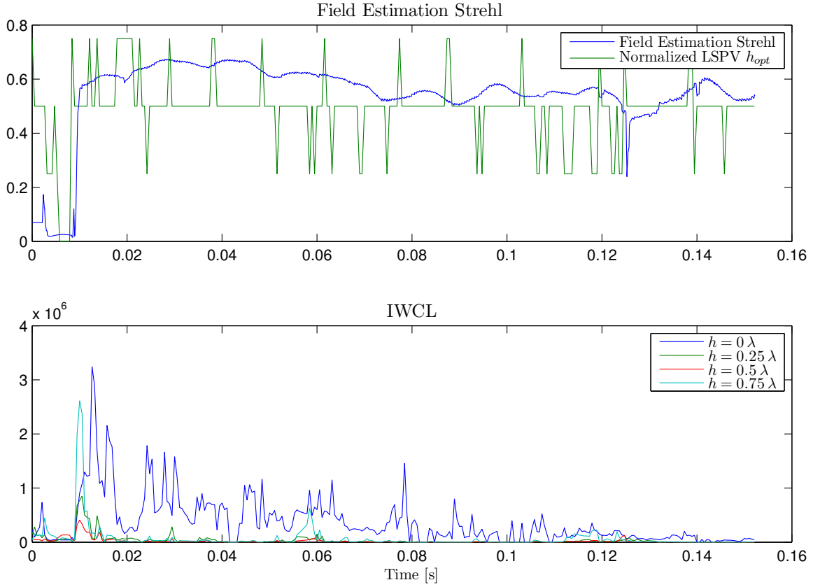
Figure 4.8: The top plot shows field estimated Strehl ratio and h_{opt} over time with an LSPV+4 reconstructor. The bottom plot shows the IWCL for each of the four \phi_{rot} realizations over the same time interval. This is in conditions of \sigma_\chi^2 = 0.5 , f_g = 40\text{Hz} , d/r_0 = 1/2 .
