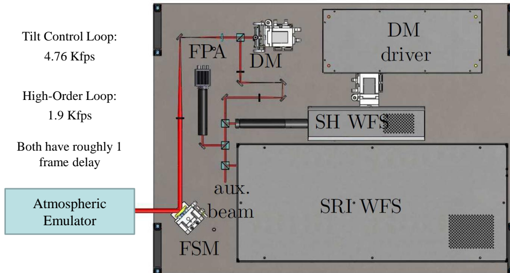
Figure 3.1: Layout of AFIT's AO system testbed.
