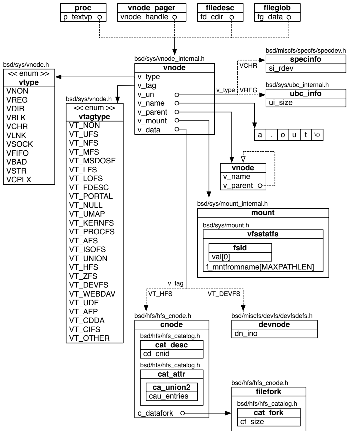
Figure 8. Virtual node (vnode).
