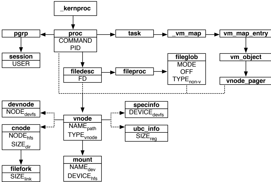
Figure 4. C struct relationship overview.
