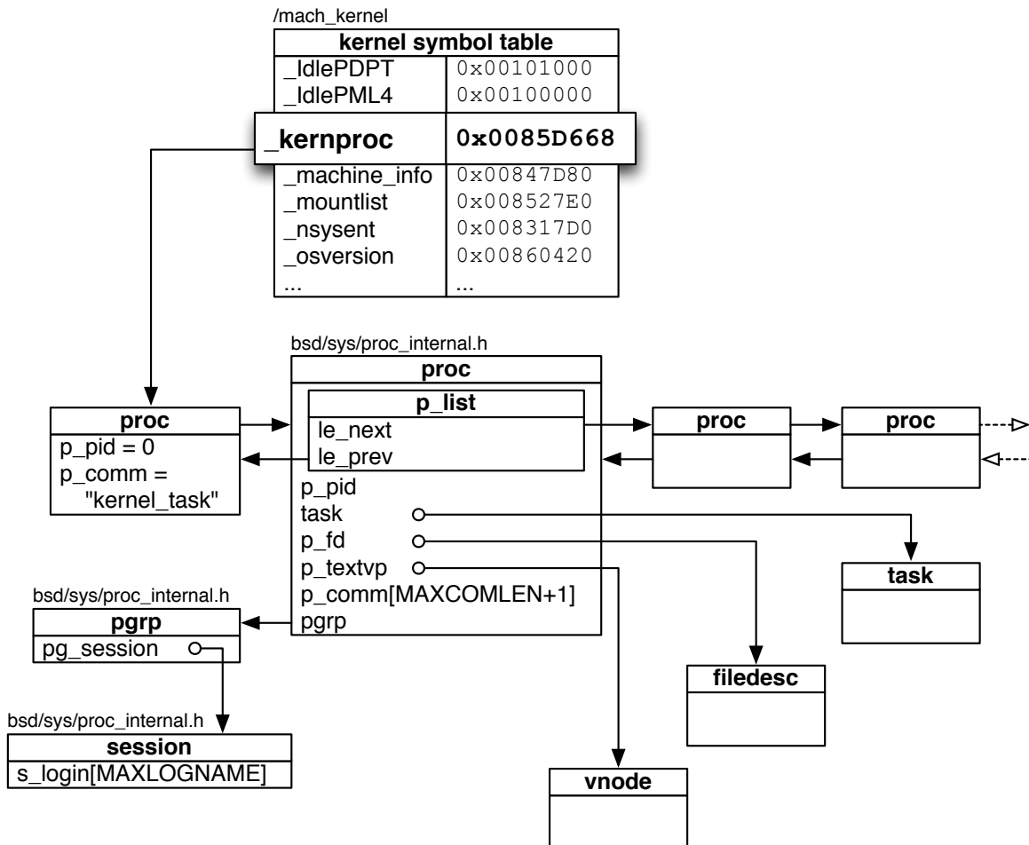
Figure 5. Symbol table and process list.
