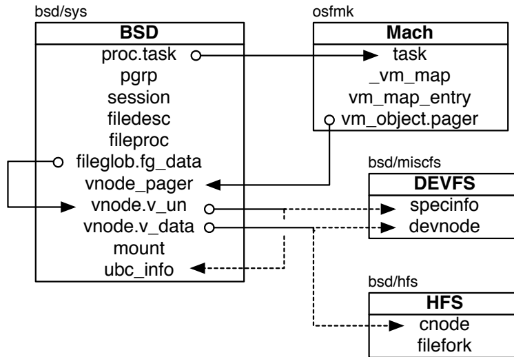
Figure 10. Abstraction crossover.
