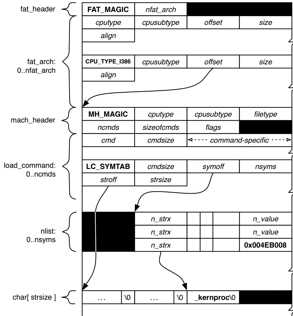
Figure 1. mach_kernel executable.
