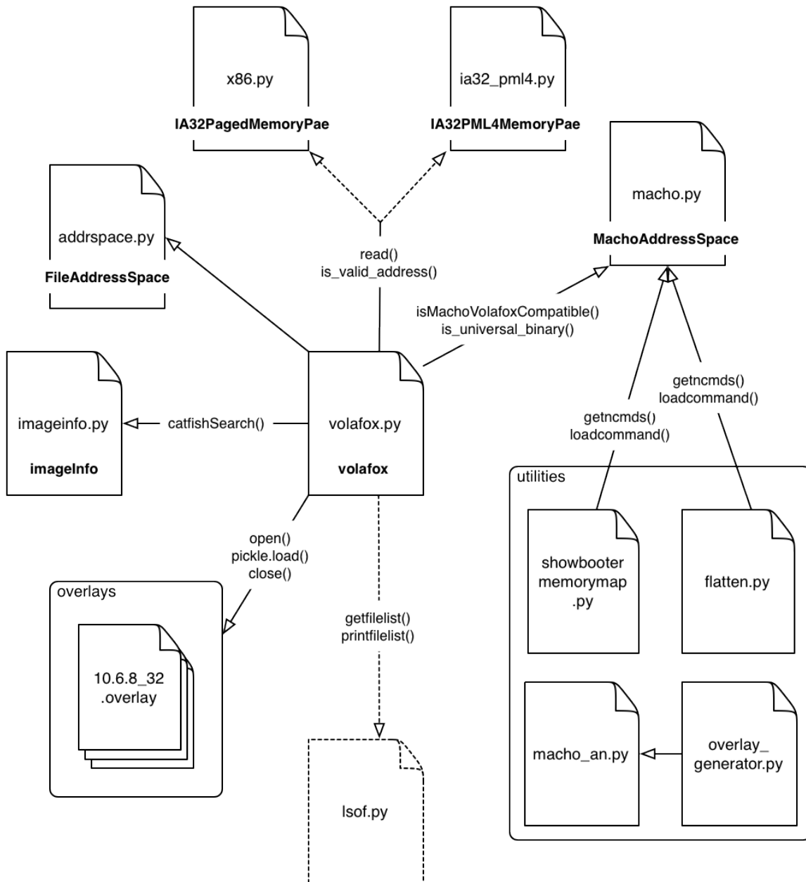
Figure 11. volafox package diagram.
