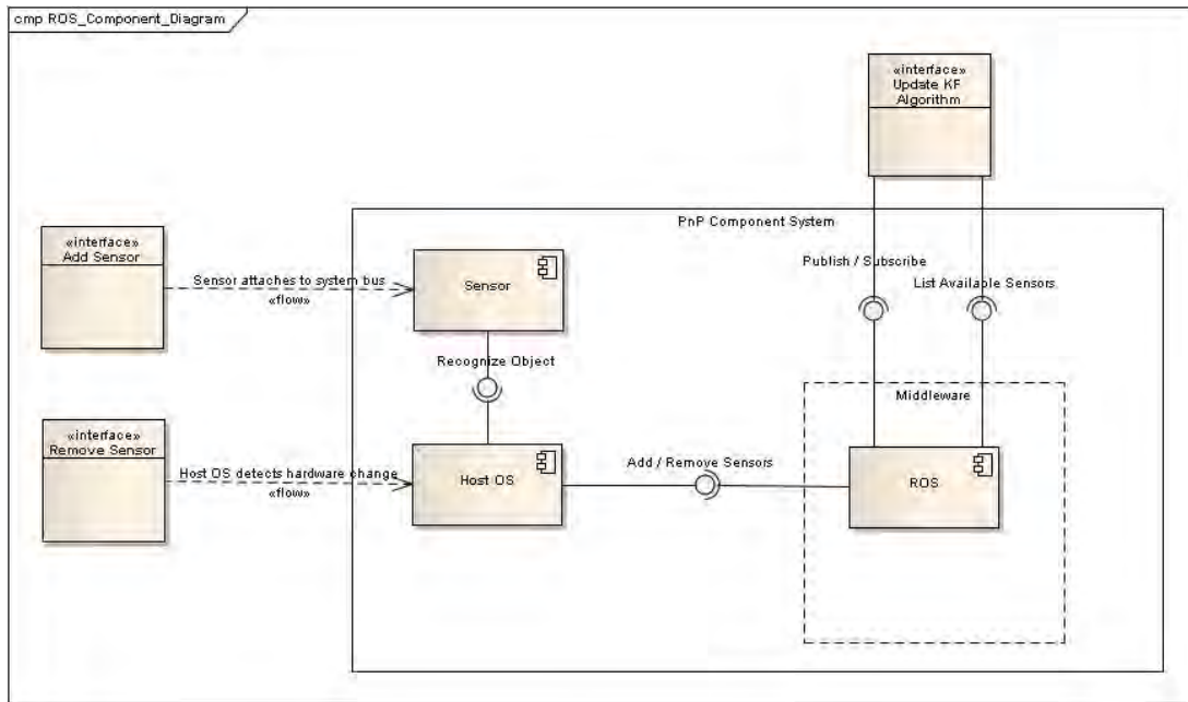
Figure III.6: ROS-centered component diagram for a PnP sensor system
