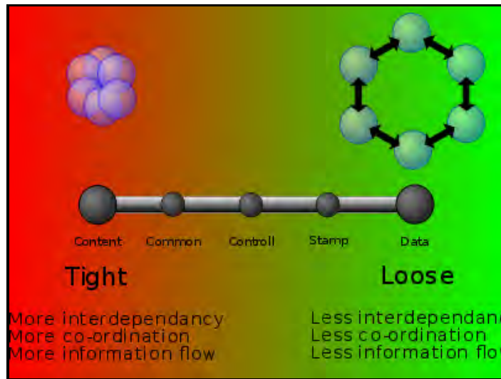
Figure IV.9: Software Coupling [51]
