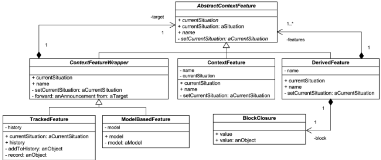
Figure II.11: ContextFeature hierarchy [10]
