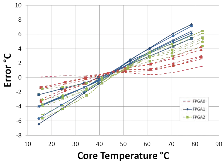
Figure 19. Digital temperature sensor response error vs System Monitor ADC across 3 FPGAs after auto calibration
