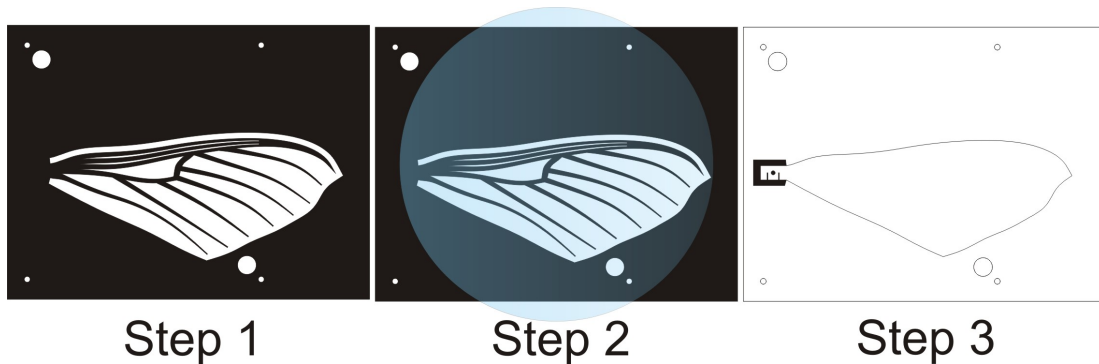
Figure 89: Venation Cutting Pattern and Venation/Membrane Release Pattern
