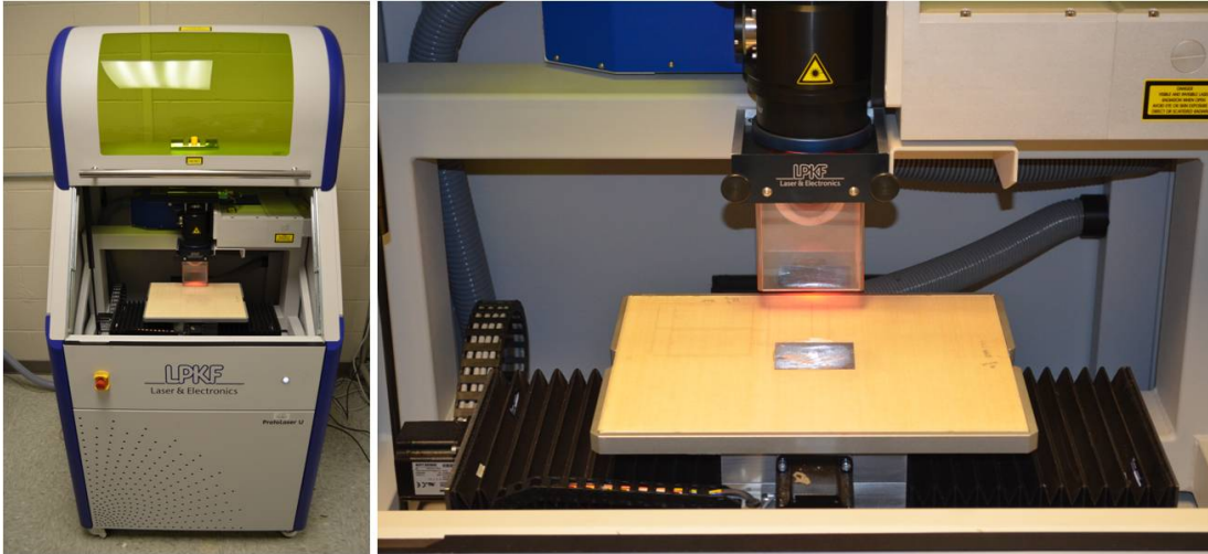
Figure 86: LPKF Protolaser U Machining Center
