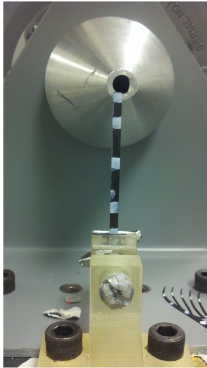
Figure 65: 40 mm x 2.5 mm beam with airhorn excitation
