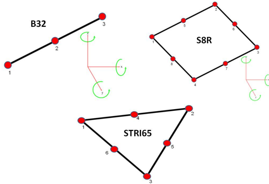
Figure 46: FEA Element Types
