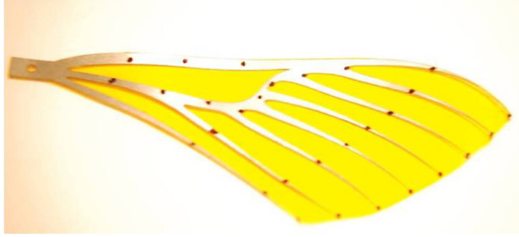
Figure 52: Laser Cut Stainless Steel Wing [17]
