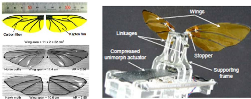
Figure 21: Hand Fabricated Uniaxial Carbon Fiber Wings [60, 61]
