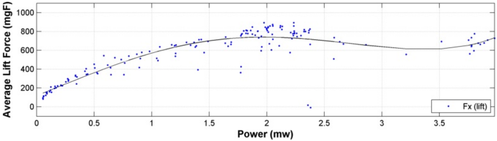
Figure 123: Baseline Engineered wing Flapping Analysis
