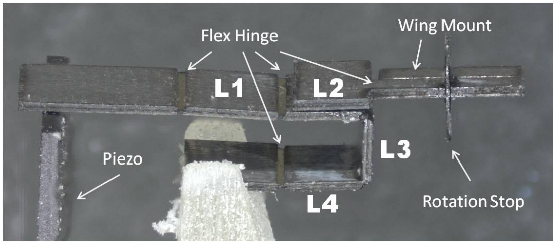
Figure 93: Fabricated Linkage Side View
