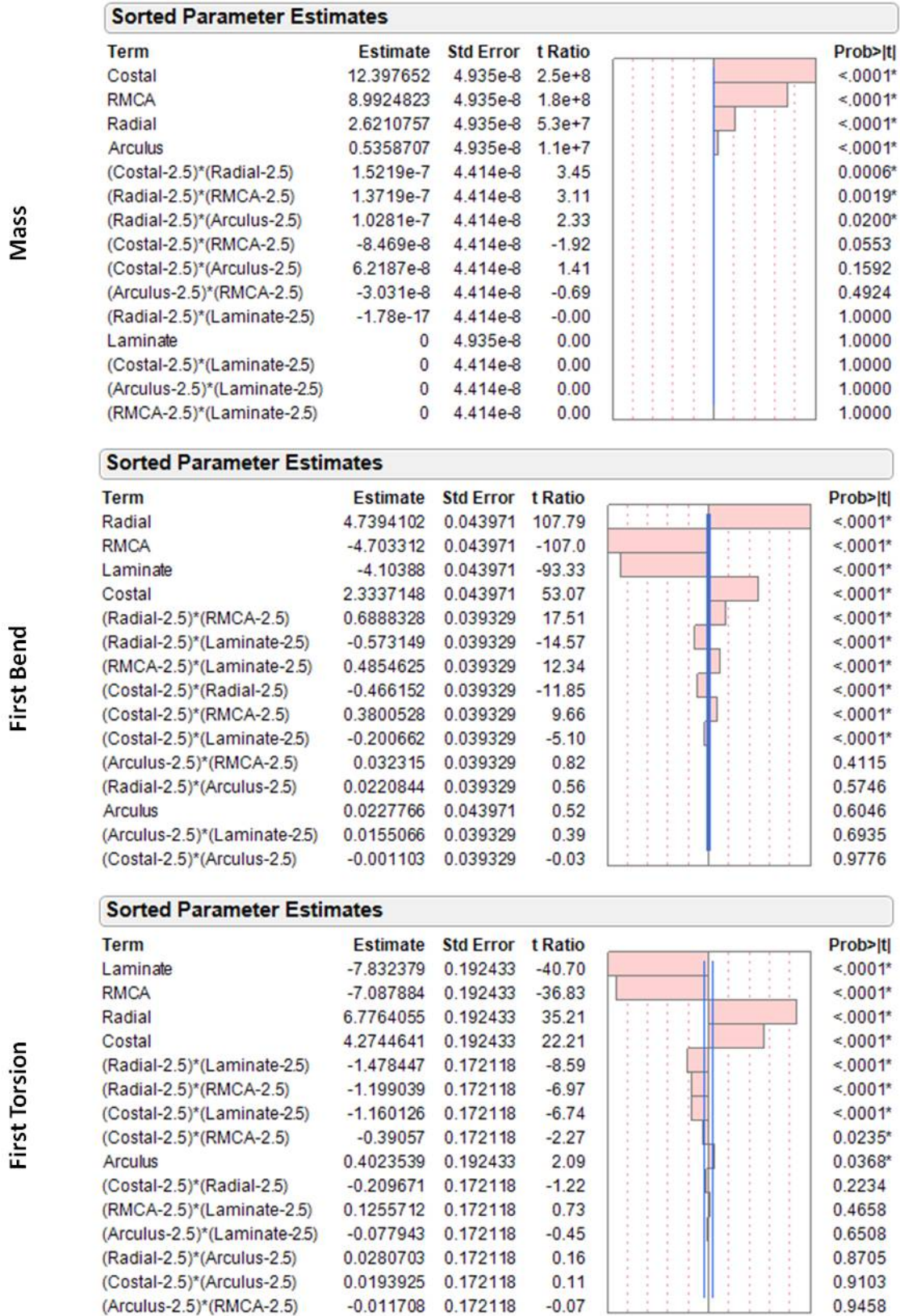
Figure 73: DOE Results Table
