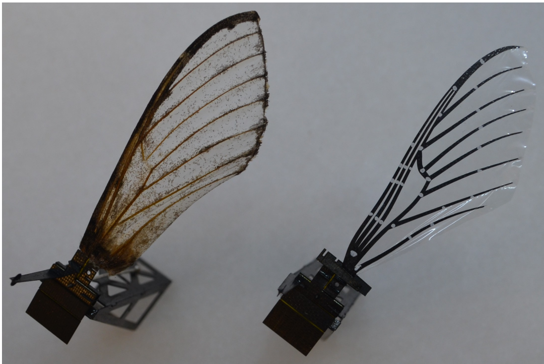
Figure 90: Biological Wing vs. Baseline Engineered Wing
