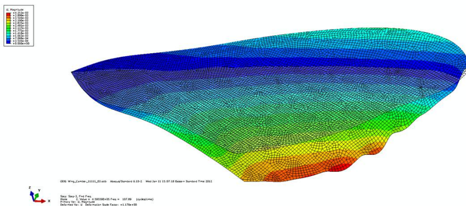
Figure 75: Engineered Wing First Torsion Modeshape
