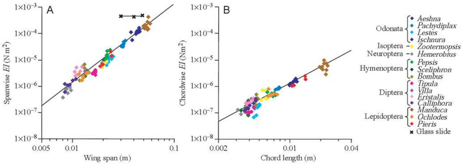
Figure 7: Flexular Wing Stiffness of Various Insect Species [12]
