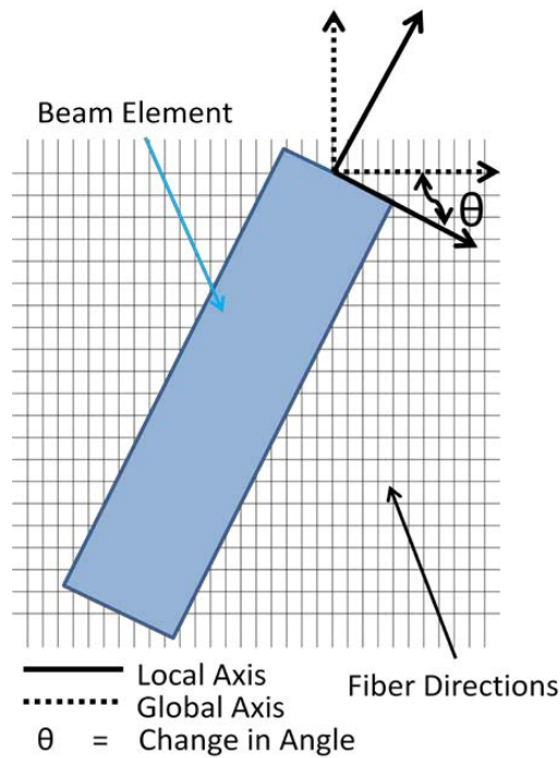
Figure 70: Global Laminate Axis vs. Local Venation Axis [90]
